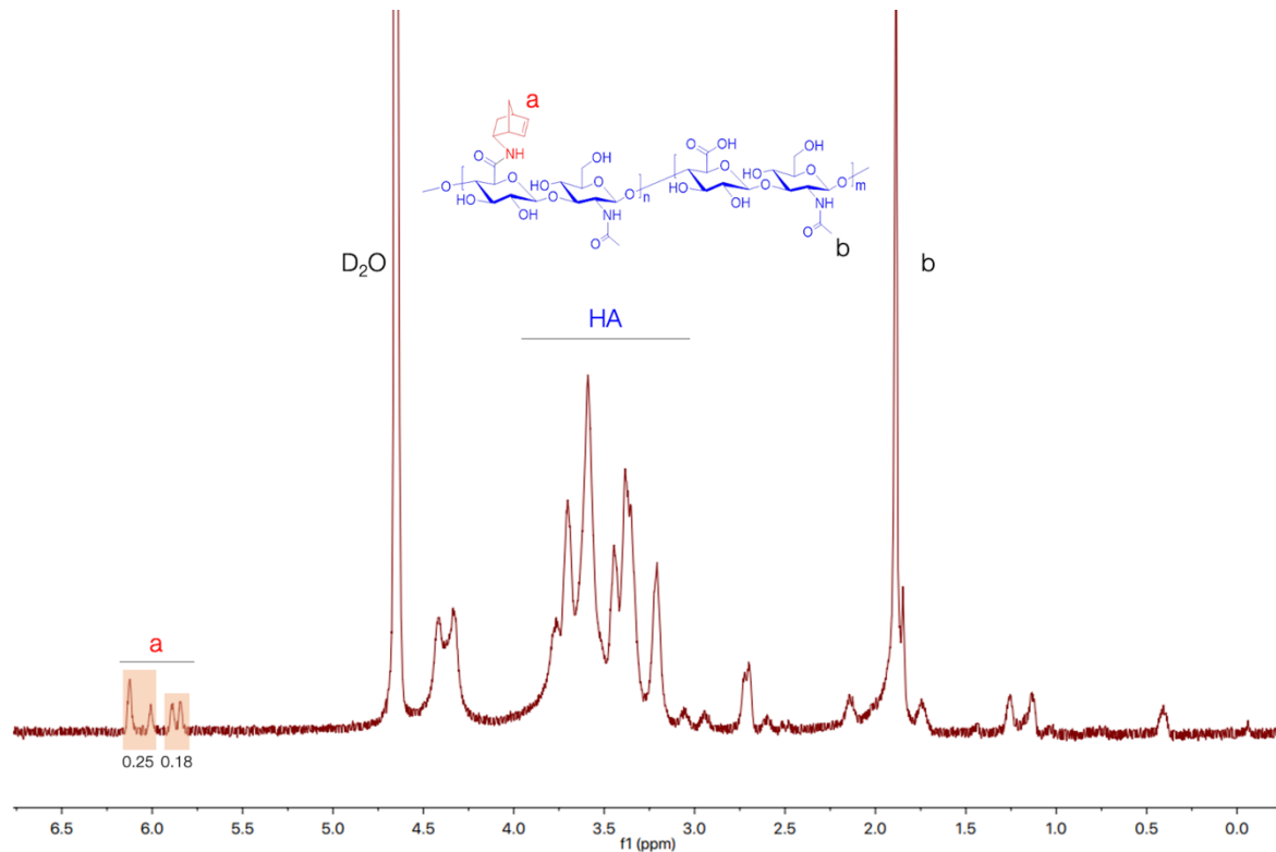
Fig. S1: ^1\text{H} NMR spectrum of norbornene-modified hyaluronic acid (NorHA). Spectrum indicates \sim 22\% modification of HA repeat units with norbornene groups.
