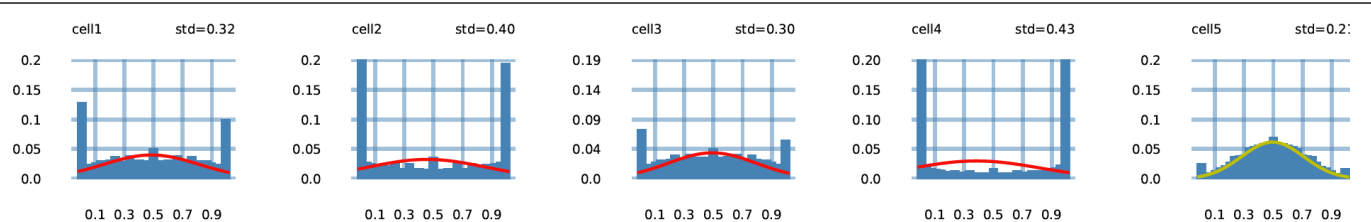
Fig S8. Allele frequency distribution of heterozygous germline variants in 5 MDA-amplified cells. Cell5 was selected for further analysis owing to its most uniform amplification and lower allele drop out as compared to the other cells.
