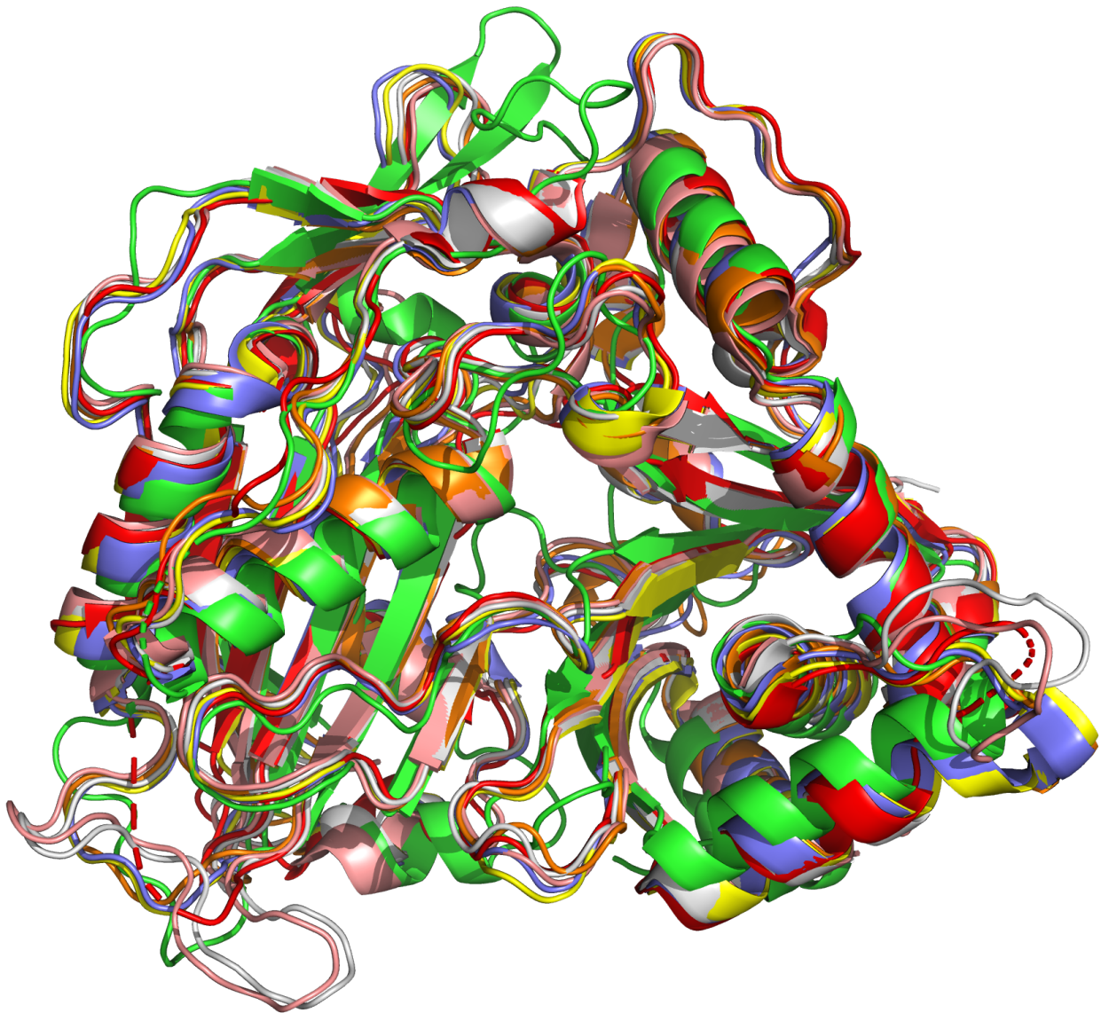
Supplementary Figure S7. Structural overlay of BOS with five homologs. The structure of BOS (green) was aligned with the structures of six hydroxycinnamoyl transferases from: Selaginella moellendorffii (PDB ID: 6DD2, red), Arabidopsis thaliana (PDB ID: 5KJU, orange), Coffea canephora (PDB ID: 4G0B, yellow), Panicum virgatum (PDB ID: 5FAL, pink), Sorghum bicolor (PDB ID: 4KE4, gray), and Plectranthus scutellarioides (PDB ID: 5KJV, purple). The figure was generated using PyMol (Molecular Graphics System, version 2.4, Schrödinger, LLC).
