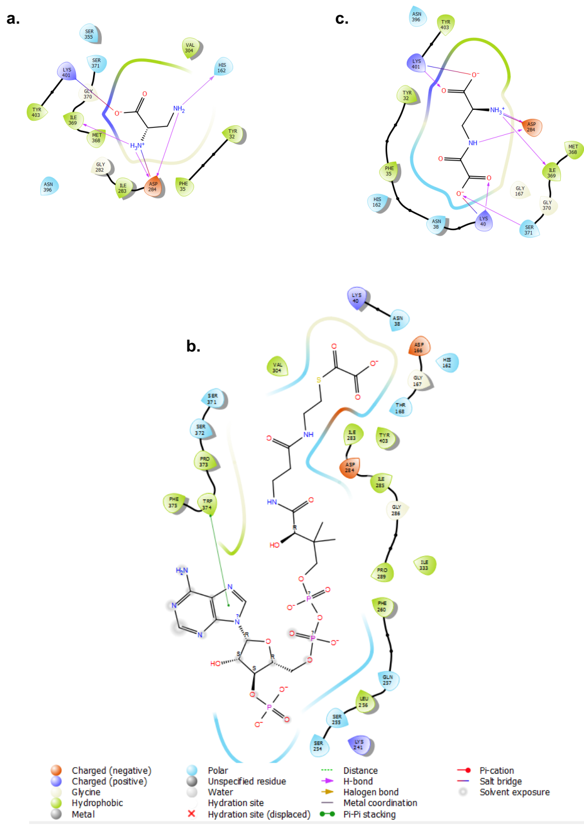
Supplementary Figure S10. Interaction maps of BOS with its ligands and product. The panels depict the interactions of BOS with L-DAPA (a), oxalyl-CoA (b) and \beta -ODAP (c). Protein-ligand interactions were derived from individual docking studies and the interaction diagrams were generated using GLIDE (Schrödinger, LLC)
