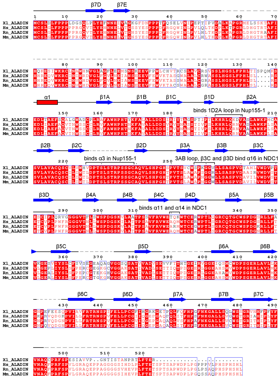
Supplementary information, Fig. S13 | Sequence alignment of ALADIN orthologues from X. laevis (XI), Homo sapiens (Hs), Rattus norvegicus (Rn), and Mus musculus (Mm).
