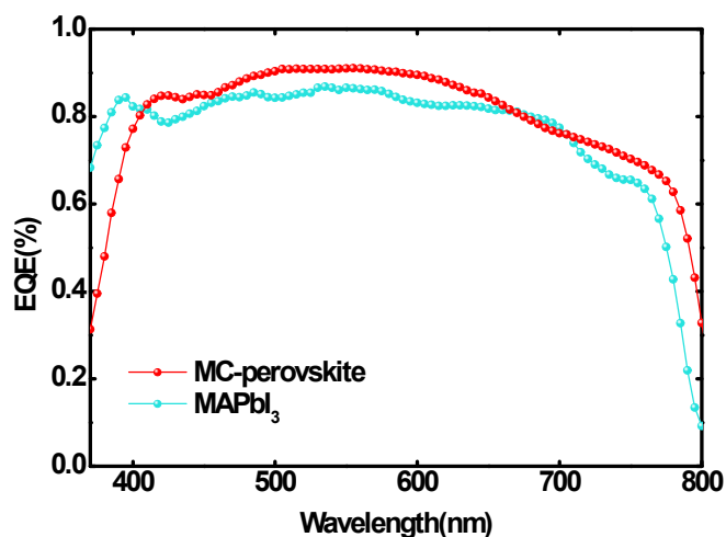
Figure S1. IPCE (EQE) of MAPbI 3 and MC-perovskite.
