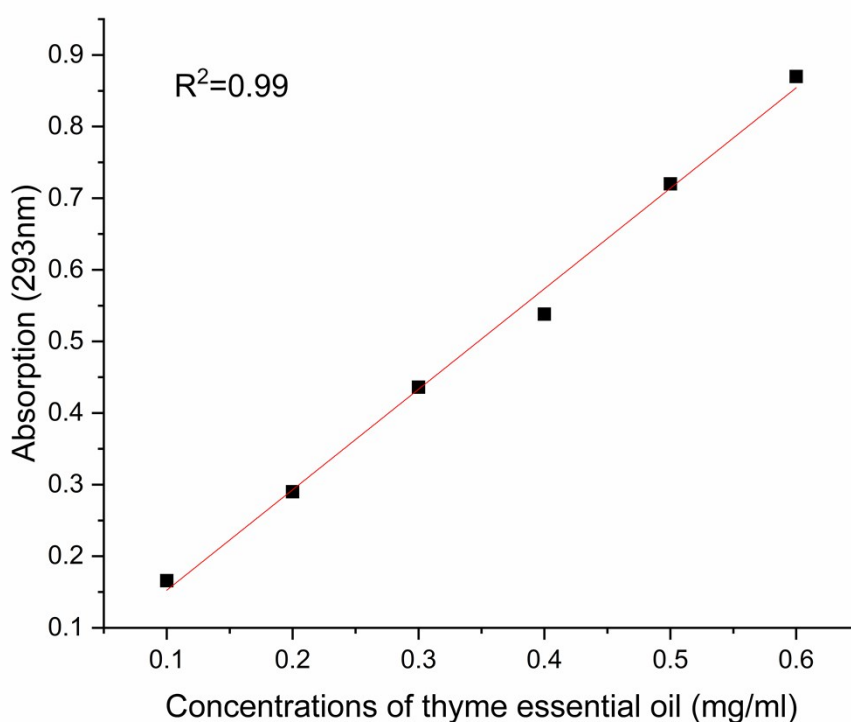
Fig. S1 Linear correlation between the absorbance values (calibration curve) for the peaks at 293 nm and the thyme essential oil concentrations in ethanol.
