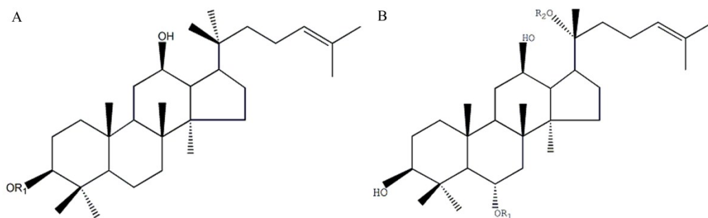
Figure 1 The chemical molecular structure of protopanaxadiol-type ginsenosides (A) and protopanaxatriol-type ginsenosides (B).
