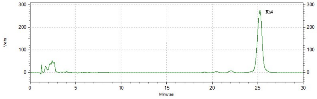
Figure 2 The standard spectrums of S-Rg3, R-Rg3, Rk1, Rg5, S-Rh1, R-Rh1, Rk3 and Rh4.
