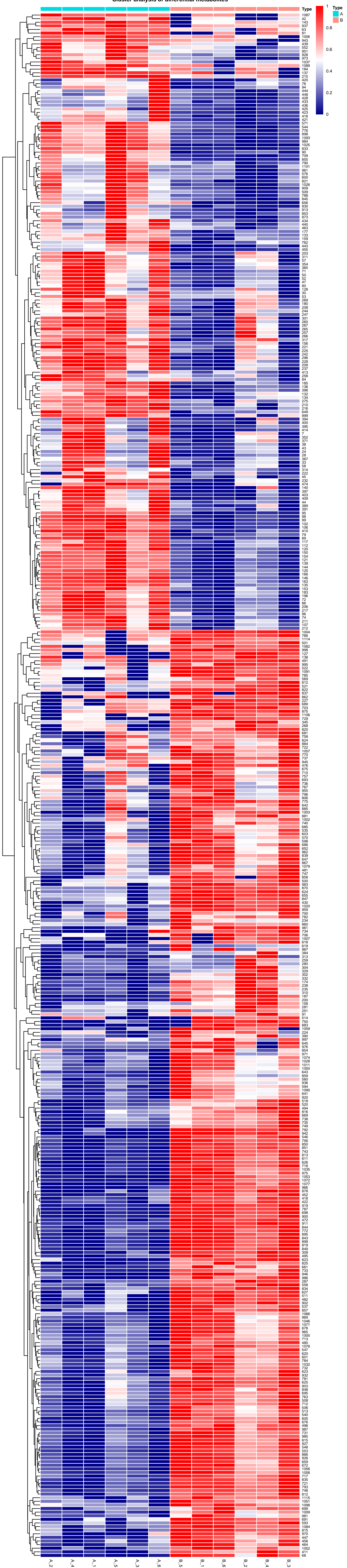
Cluster analysis of differential metabolites
