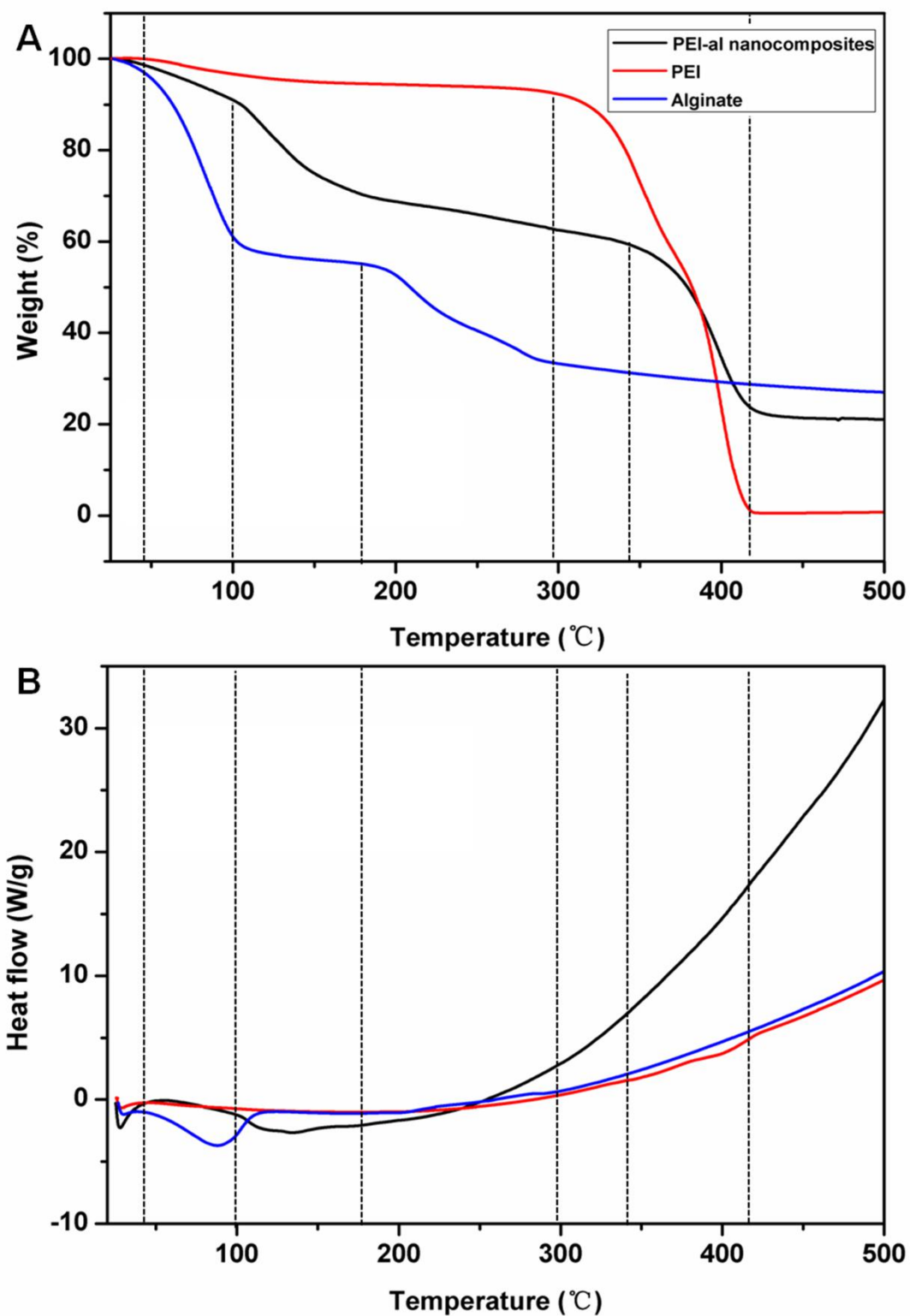
Figure S1: Thermal properties of PEI-al nanocomposites, PEI and alginate. (A) TGA curves. (B) DSC curves.
