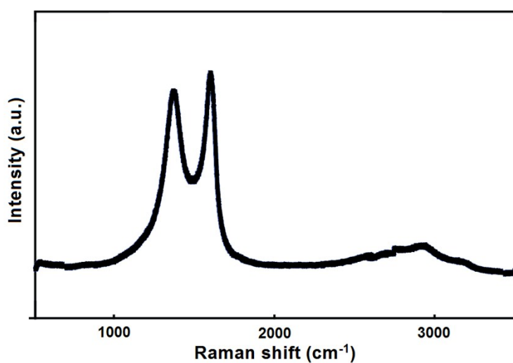
Fig. S1: The Raman spectrum of prGO.
