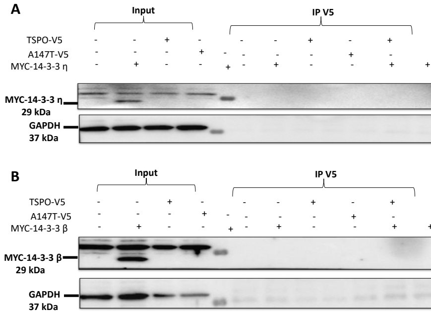
Fig S1. Validated non-interactors of hTSPO WT and hTSPO A147T . A-B) 14-3-3 \eta protein (YWHAH) and 14-3-3 \beta (YWHAB) were expressed in U87MG cells together with V5-tagged human TSPO WT or TSPO A147T . A) Co-IP of YWHAH and hTSPO WT or hTSPO A147T with V5 antibody and detected by immunoblotting for myc. YWHAH was not co-purified with V5. B) Co-IP of YWHAB and hTSPO WT or hTSPO A147T with V5 antibody and detected by immunoblotting for myc. YWHAB was not co-purified with V5.
