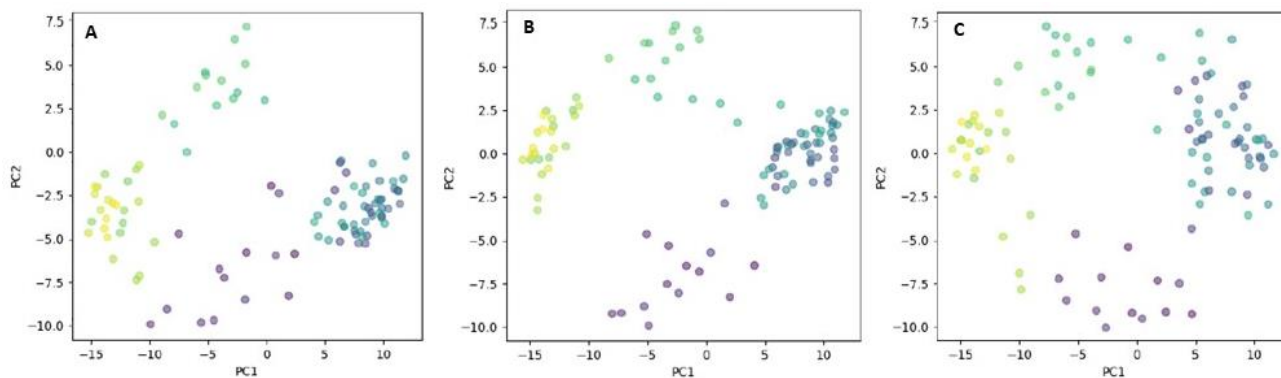
Figure S1. PCA plots of apo-IFN simulations.
