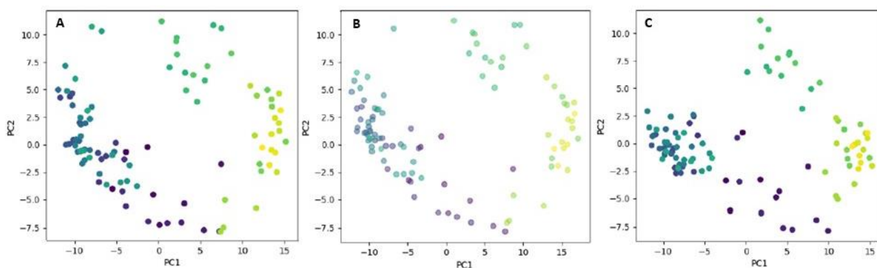
Figure S2. PCA plots of PEG200-IFN simulations.
