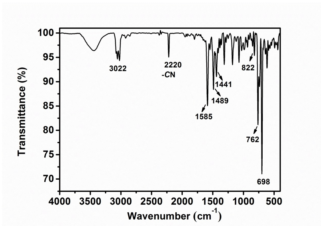
Fig. S4 FT-IR spectrum of B-TPEAN.
