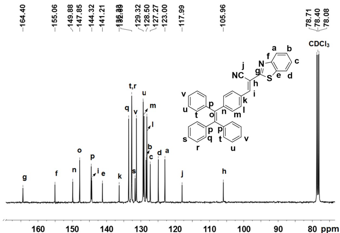
Fig. S2 13 C-NMR spectrum of B-TPEAN.
