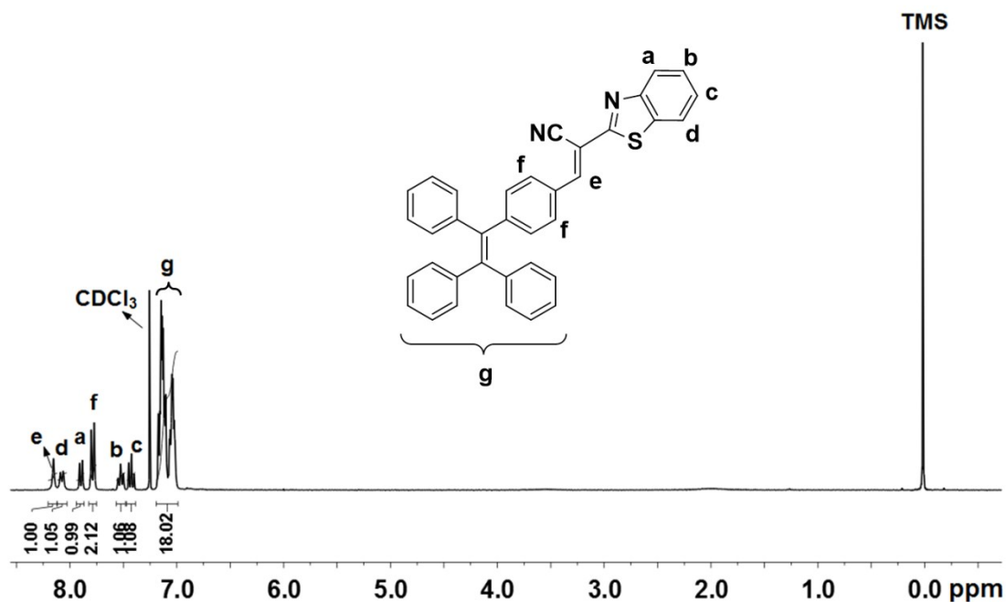
Fig. S1 1 H-NMR spectrum of B-TPEAN.
