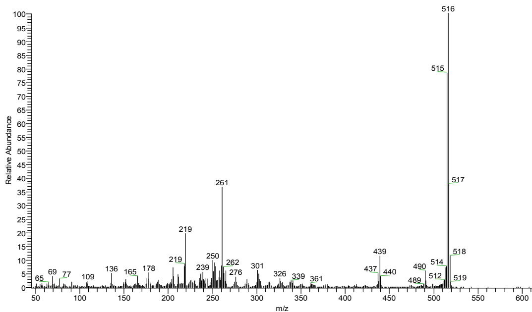
Fig. S3 MS spectrum of B-TPEAN.
