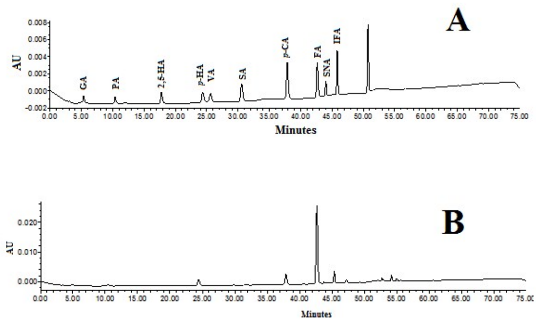
Fig 1 the HPLC chromatogram of phenolic acid standards (A) and sample (B)
