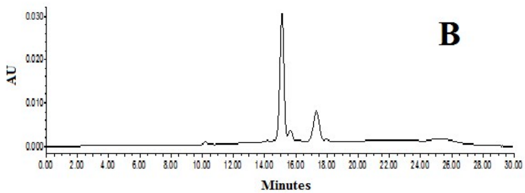
Fig 2 the HPLC chromatogram of anthocyanin standards (A) and sample (B)
