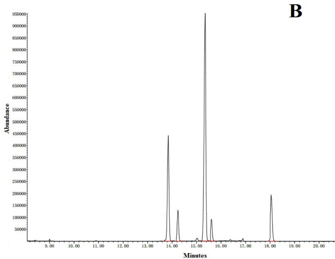
Fig 3 the GC-MS chromatogram of sterol standards (A) and sample (B)
