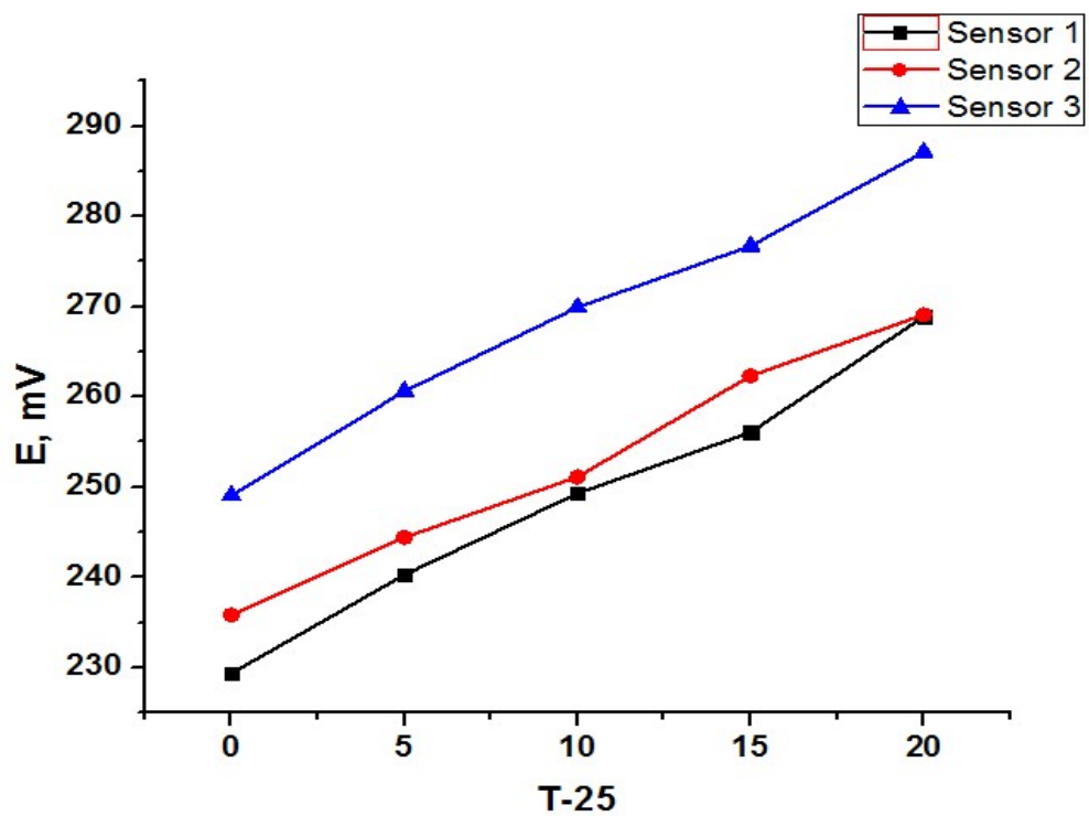
Figure (S2): Variation of standard electrode potential with changes of test solution temperatures for different SPEs.
