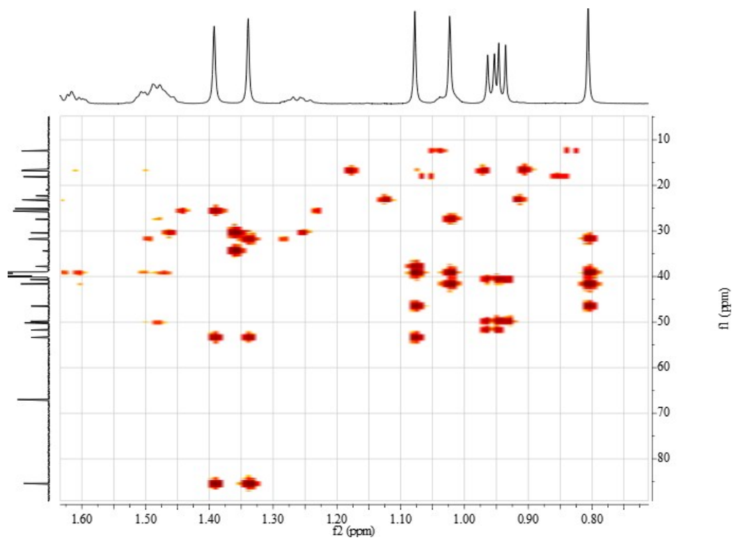
Appendix 2-7. HMBC spectrum of compound 2.
