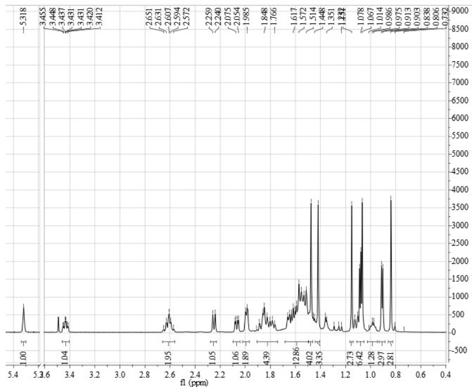
Appendix 4-2. 1 H-NMR spectrum of compound 4.
