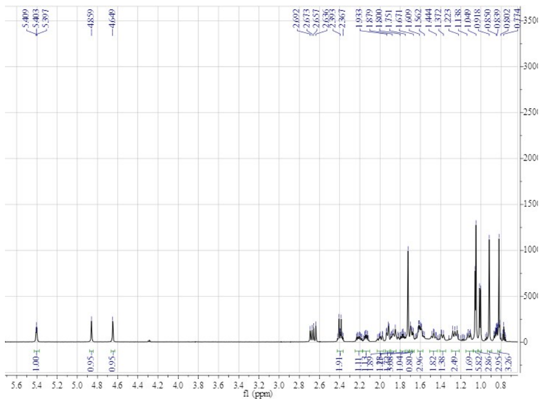
Appendix 3-2. 1 H-NMR spectrum of compound 3.
