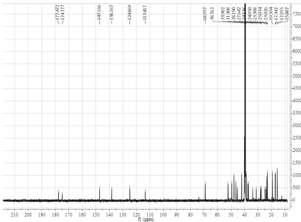
Appendix 5-3. ^{13}\text{C} -NMR spectrum of compound 5 .
