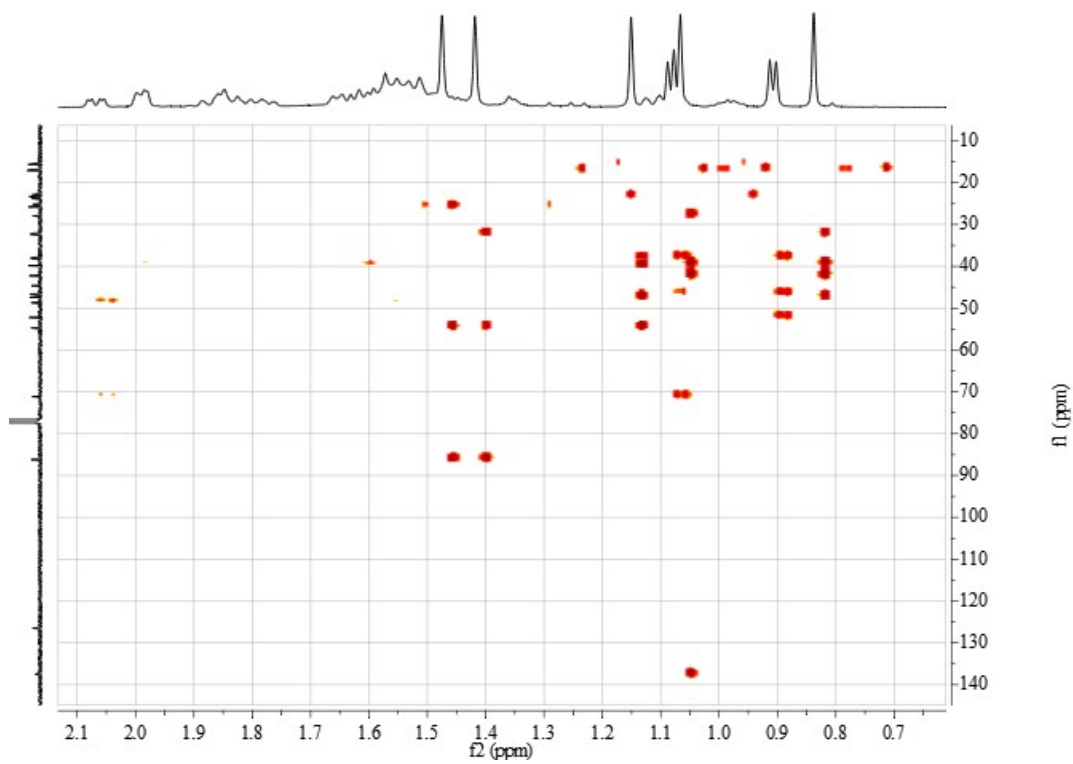
Appendix 4-5. HMBC spectrum of compound 4.
