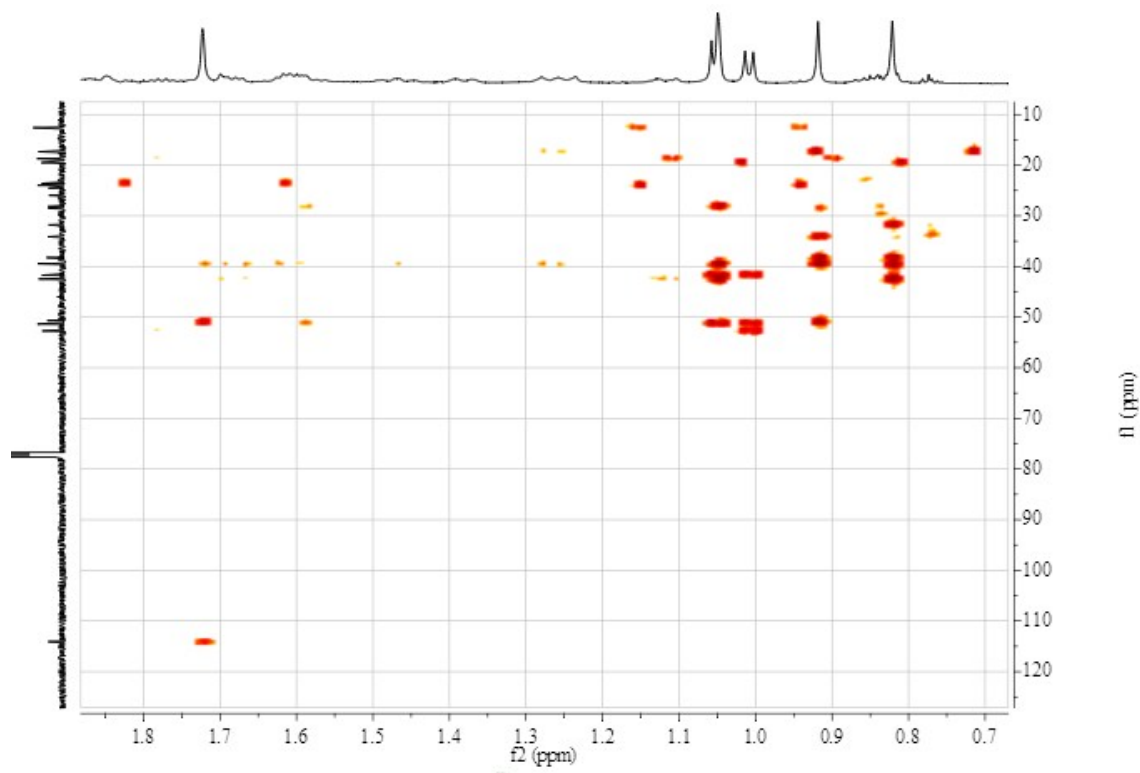
Appendix 3-6. HMBC spectrum of compound 3.
