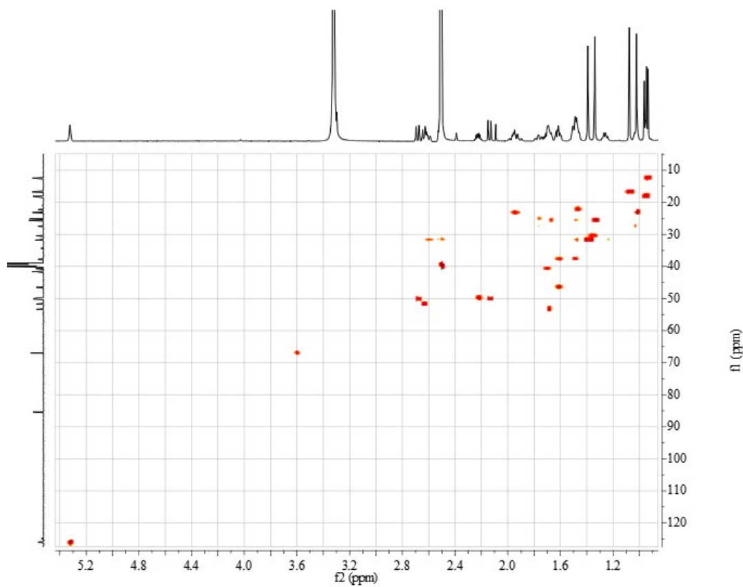
Appendix 2-5. HMBC spectrum of compound 2 .
