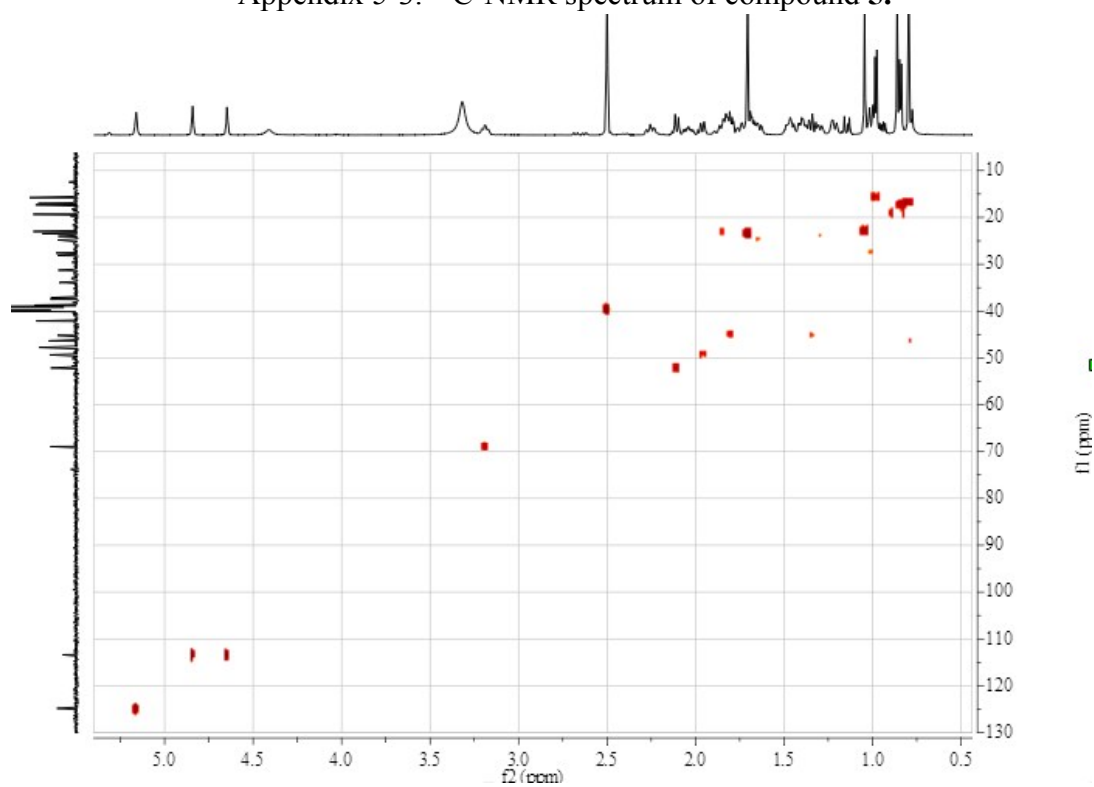
Appendix 5-4. HMQC spectrum of compound 5 .
