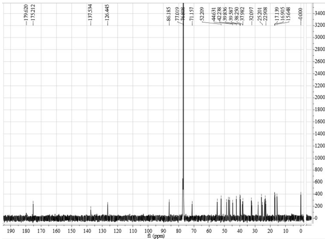
Appendix 4-3. 13 C-NMR spectrum of compound 4.
