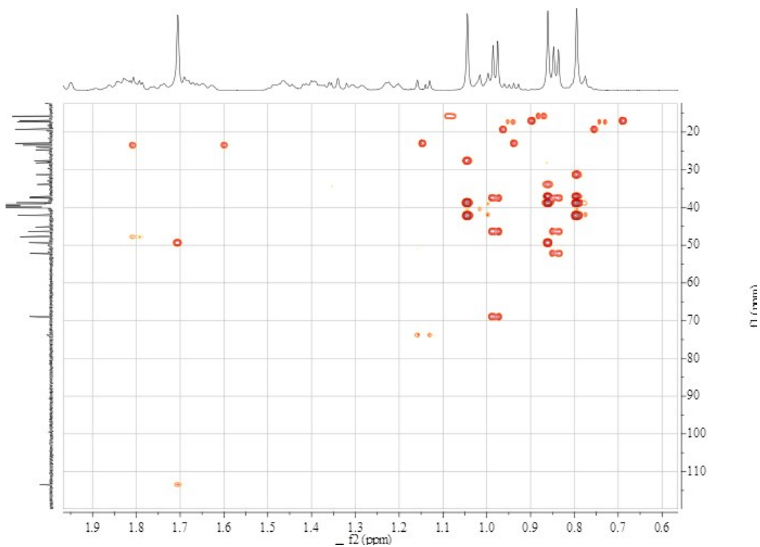
Appendix 5-6. HMBC spectrum of compound 5 .
