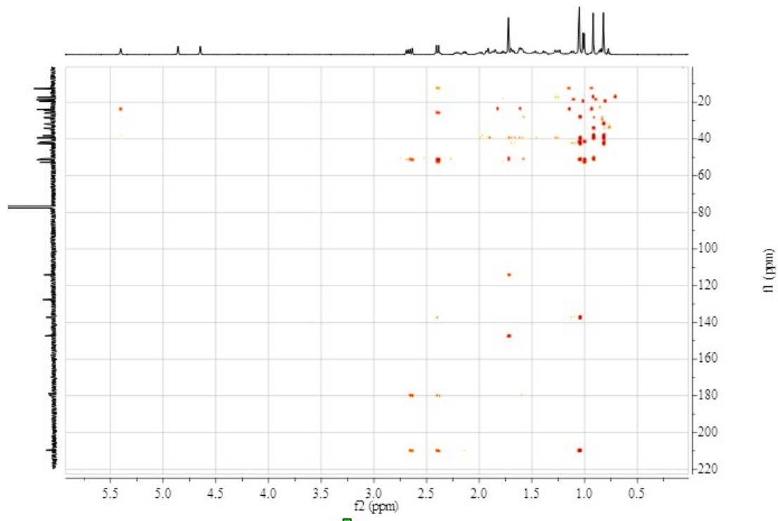
Appendix 3-5. HMBC spectrum of compound 3.
