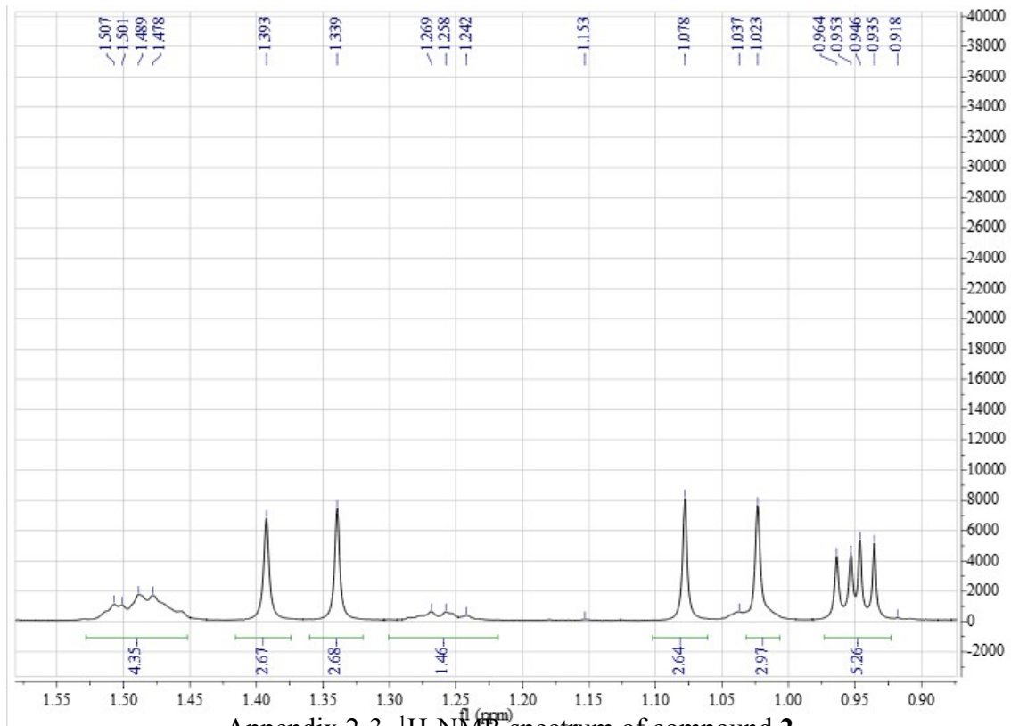
Appendix 2-3. ^1\text{H} -NMR spectrum of compound 2 .
