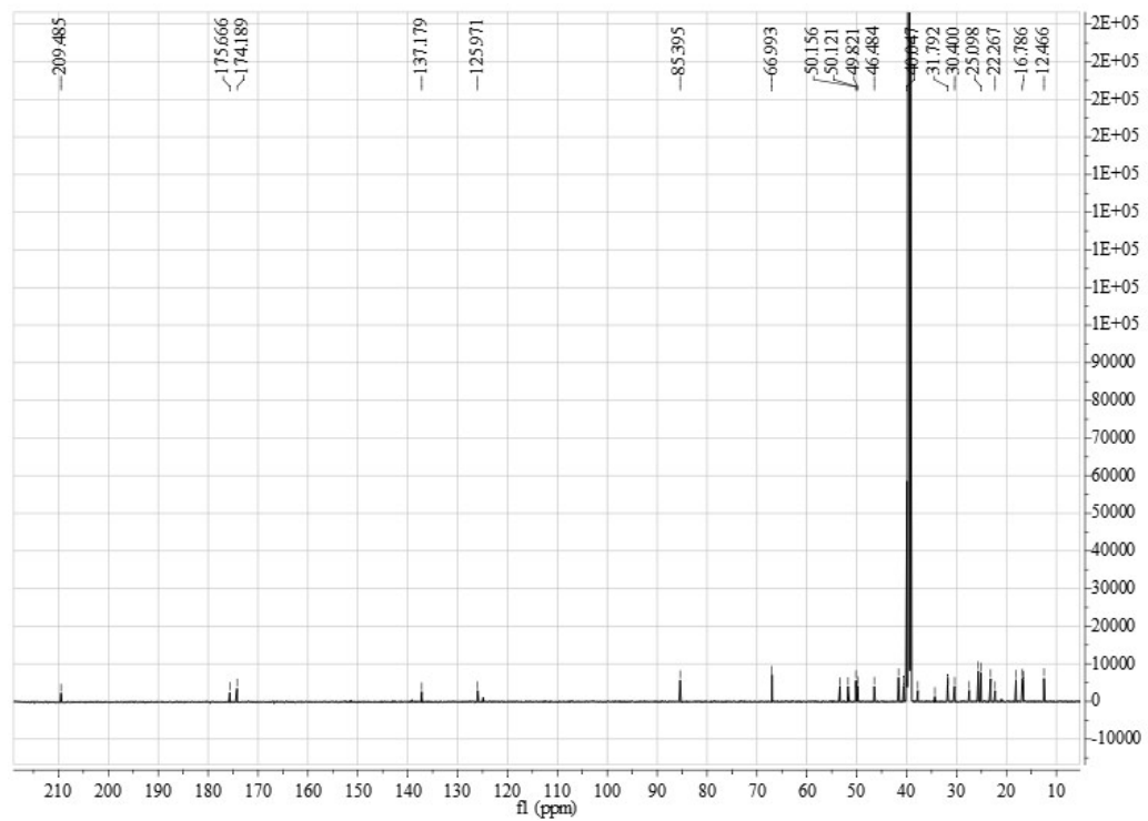
Appendix 2-4. ^{13}\text{C} -NMR spectrum of compound 2 .
