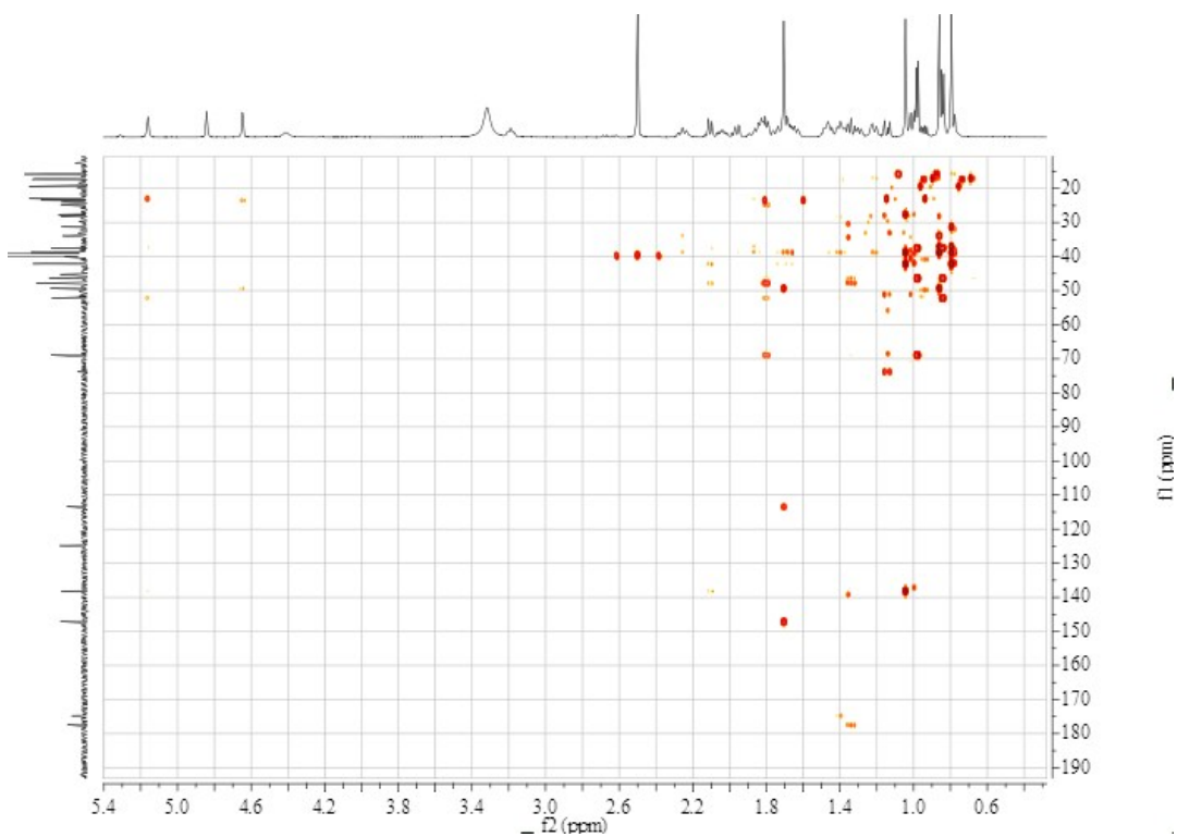
Appendix 5-5. HMBC spectrum of compound 5 .
