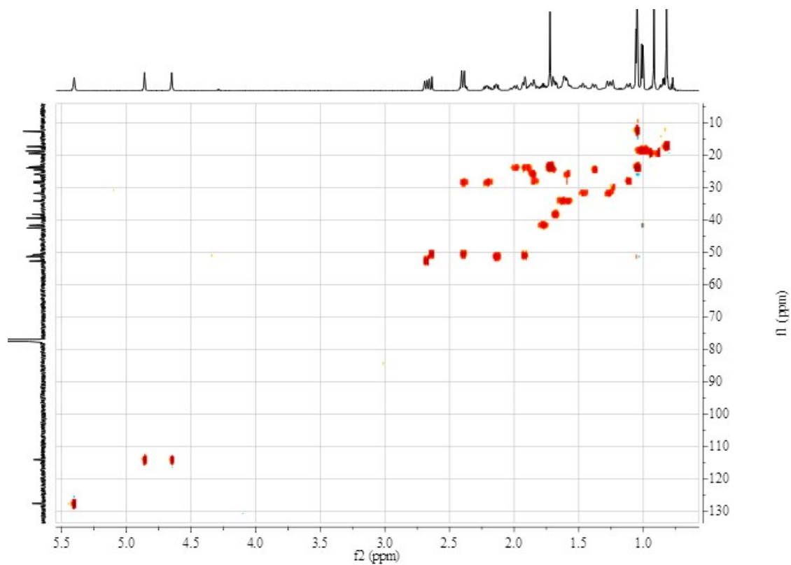
Appendix 3-4. HMQC spectrum of compound 3.
