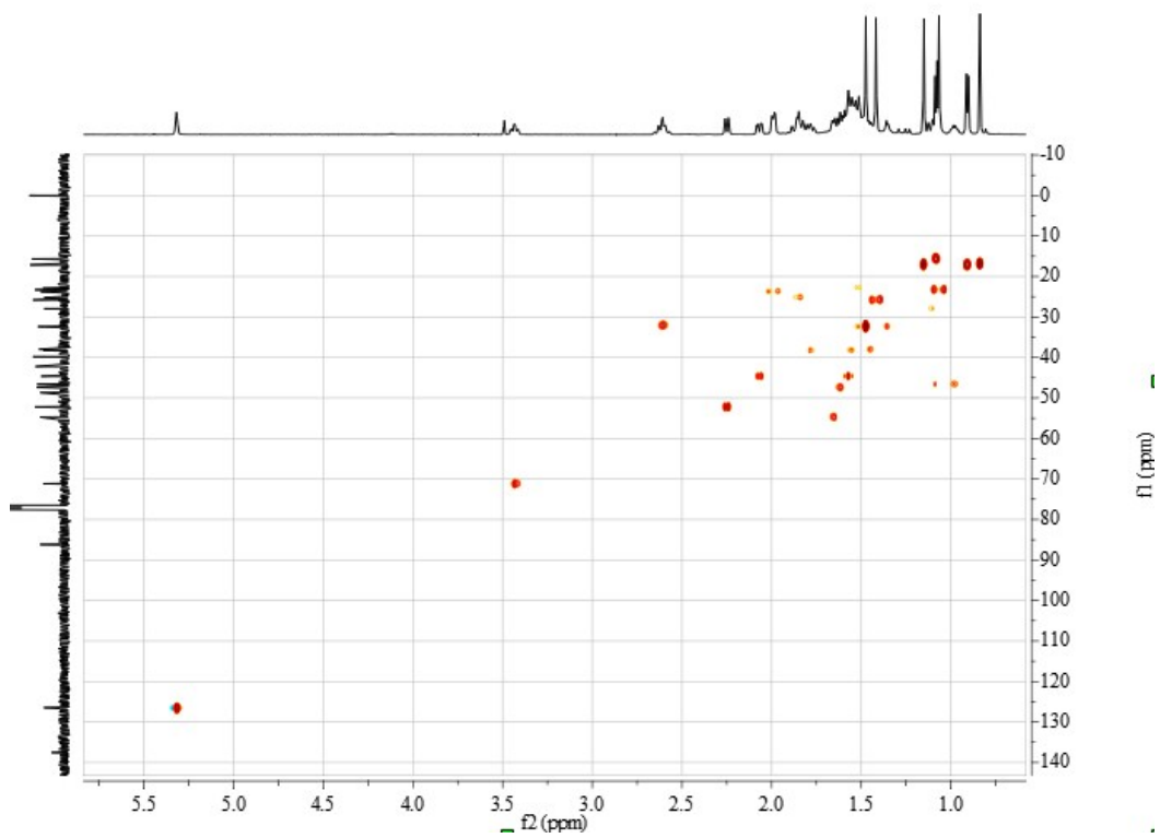
Appendix 4-4. HMBC spectrum of compound 4.
