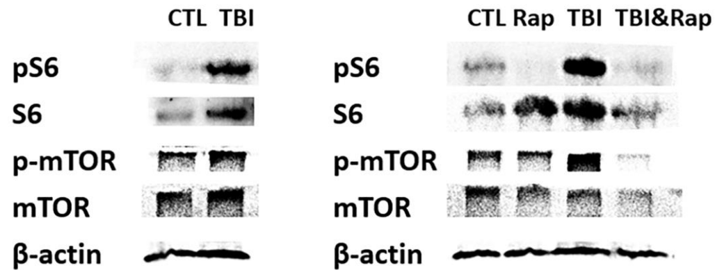
Supplementary Figure 1. Repeated experiment for main Figure 3A and C: expression of p-S6, S6, p-mTOR and mTOR after irradiation in the absence and presence of rapamycin.
