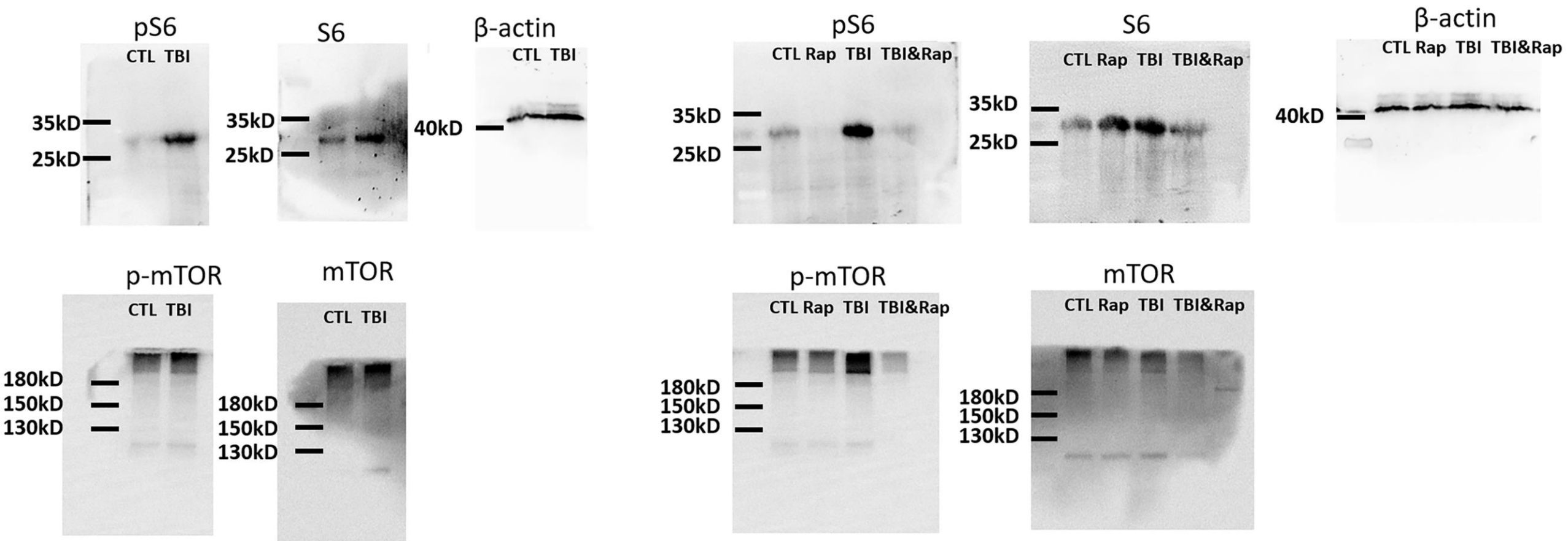
Supplementary Figure 2. Complete SDS-PAGE gels for panels shown in Supplementary Figure 1.
