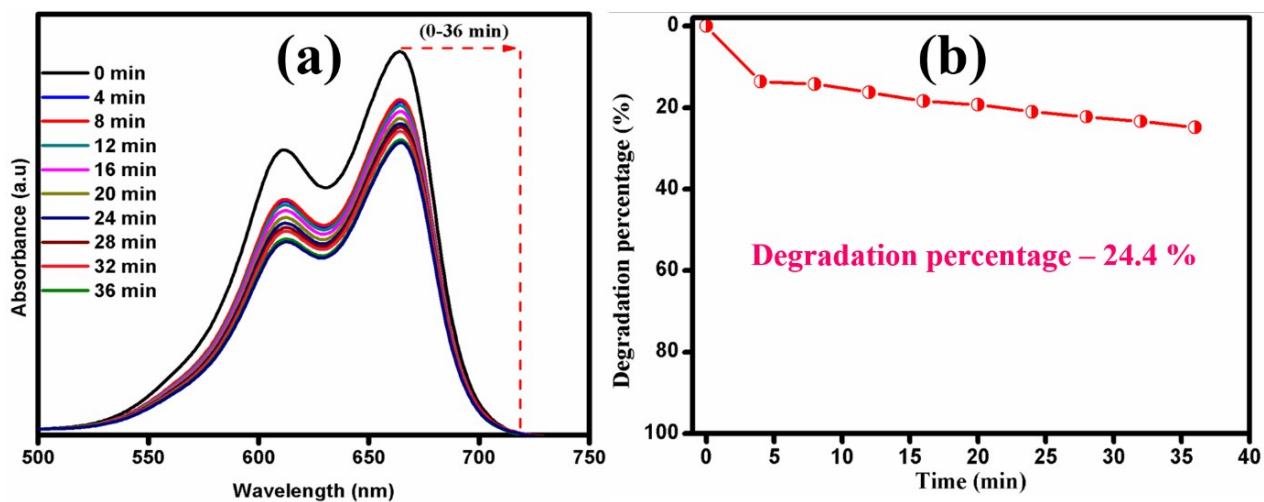
ES2. (a) Time dependent of UV-Vis absorbance spectra of MB degradation of catalyst \text{TiO}_2 , (b) Maximum degradation percentage of MB of \text{TiO}_2 catalyst.
