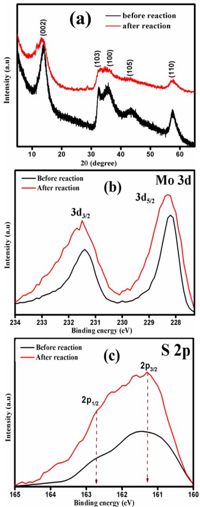
ES1 (a) XRD pattern of the sample S1 before and after the photocatalytic reaction (b) XPS spectra of sample S1 before and after degradation reaction.
