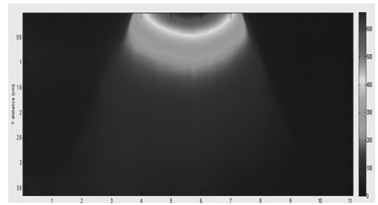
A B Supplementary Fig. 1. The percent depth dose (PDD) of applicator (A) and longitudinal central axis dose distribution of IORT (B). IORT, intraoperative radiotherapy.
