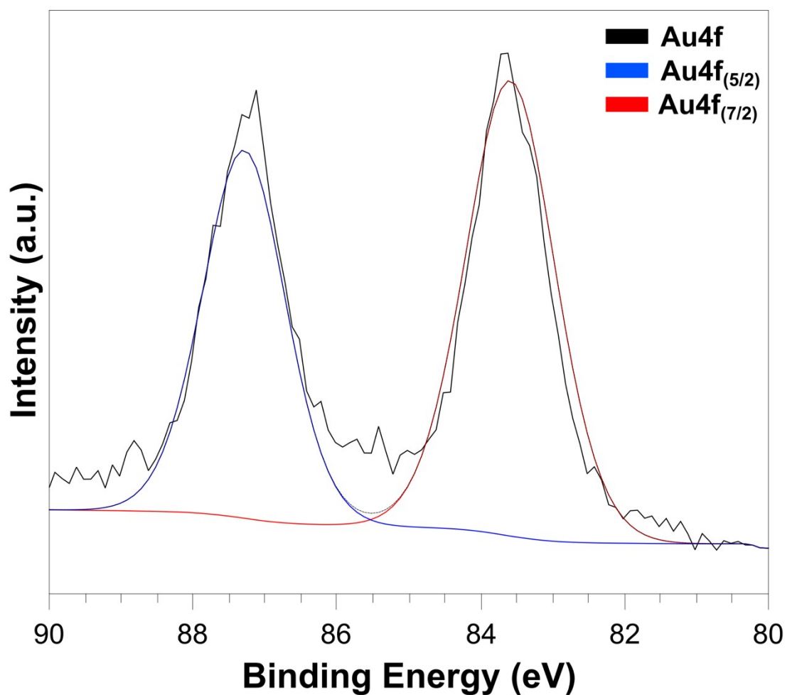
Figure 1S: XPS of AuNPs after swell encapsulation into polyurethane. The Au4f peaks confirm the presence of AuNPs into the polymer.
