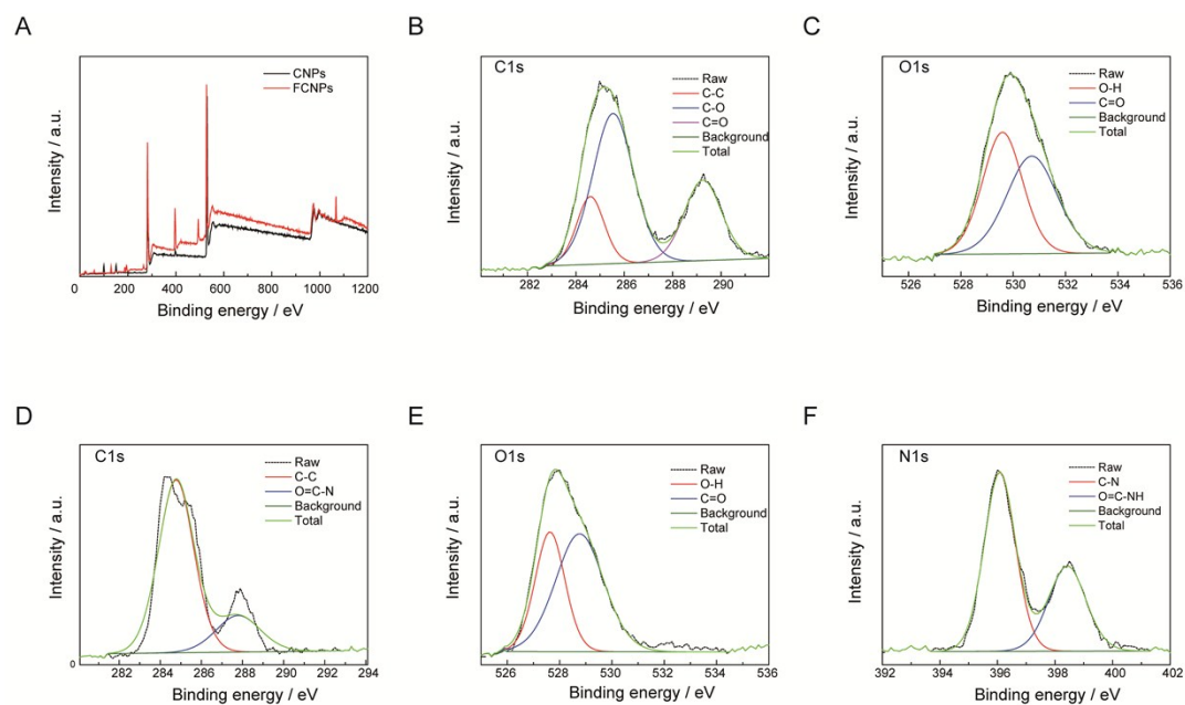
Fig. S2. XPS spectra analysis of CNPs and FCNPs. (A) XPS spectra of CNPs and FCNPs. (B ,C) CNPs high resolution peaks for C1s and O1s. (D, E and F) FCNPs high resolution peaks for C1s, O1s and N1s.
