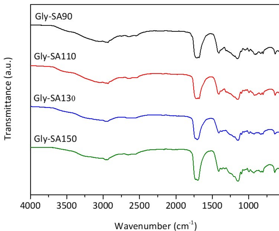
Fig. S1 FTIR spectra of Gly-SA crosslinkers.
