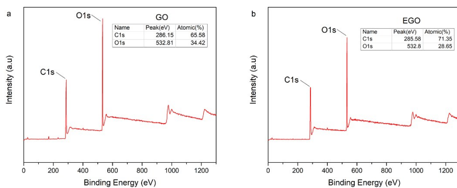
Figure S1. XPS spectra of (a) GO, (b) EGO.
