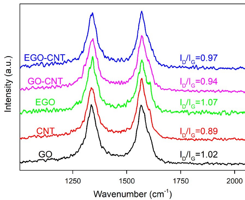
Figure S2 The Raman spectra of GO, CNT, EGO, GO-CNT and EGO-CNT.
