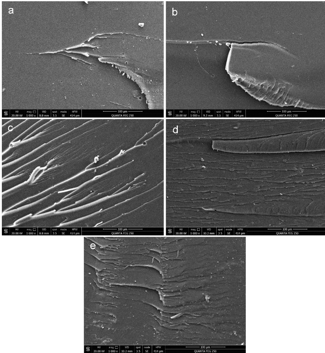
Figure S3 SEM images of fracture surfaces of SENB samples: (a) CNT/EP, (b) GO/EP, (c) EGO/EP, (d) GO-CNT/EP, (e) EGO-CNT/EP, respectively. The crack propagation direction is from left to right.
