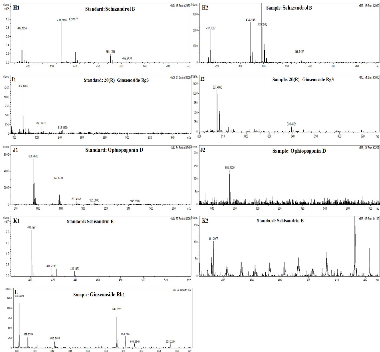
Fig. Spectrum for standards (A1) to (K1) and sample (A2) to (L).
