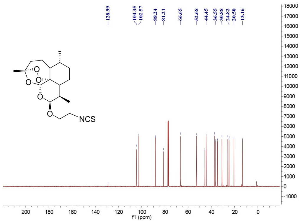
Figure S16. ^{13}\text{C} NMR spectrum of compound 5a
