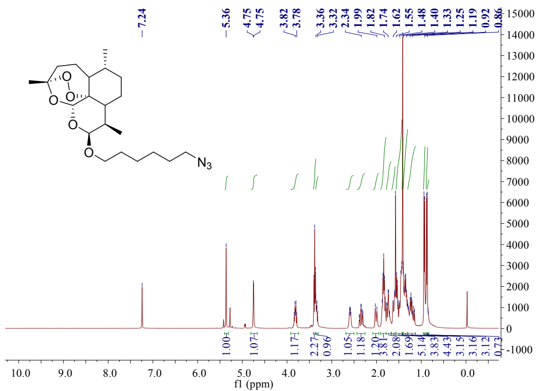
Figure S8. ^1\text{H} NMR spectrum of compound 3c
