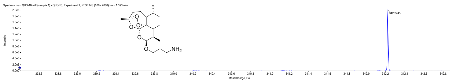
Figure S22. HR-ESI-MS of compound 4b
