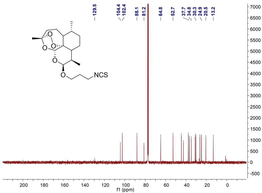
Figure S18. 13 C NMR spectrum of compound 5b
