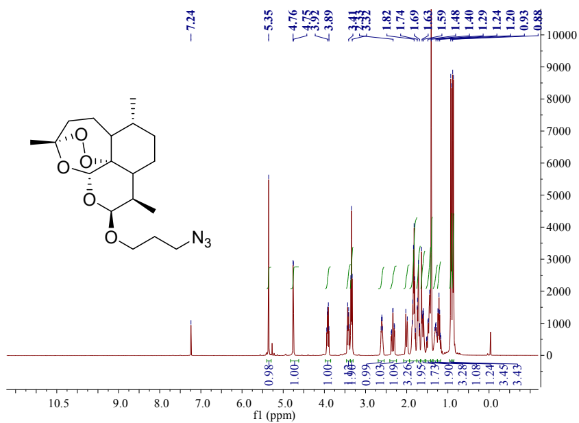
Figure S6. 1 H NMR spectrum of compound 3b
