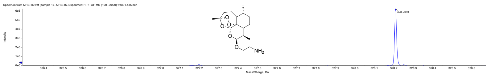
Figure S21. HR-ESI-MS of compound 4a
