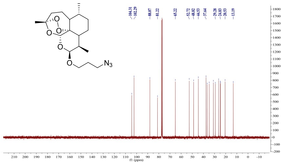
Figure S7. ^{13}\text{C} NMR spectrum of compound 3b
