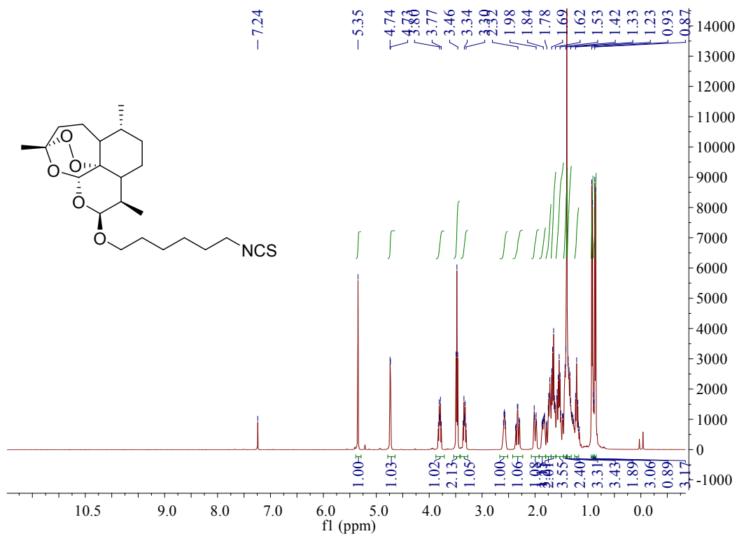
Figure S19. ^1\text{H} NMR spectrum of compound 5c
