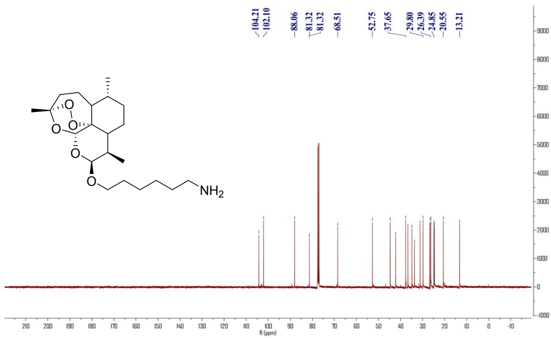
Figure S14. 13 C NMR spectrum of compound 4c
