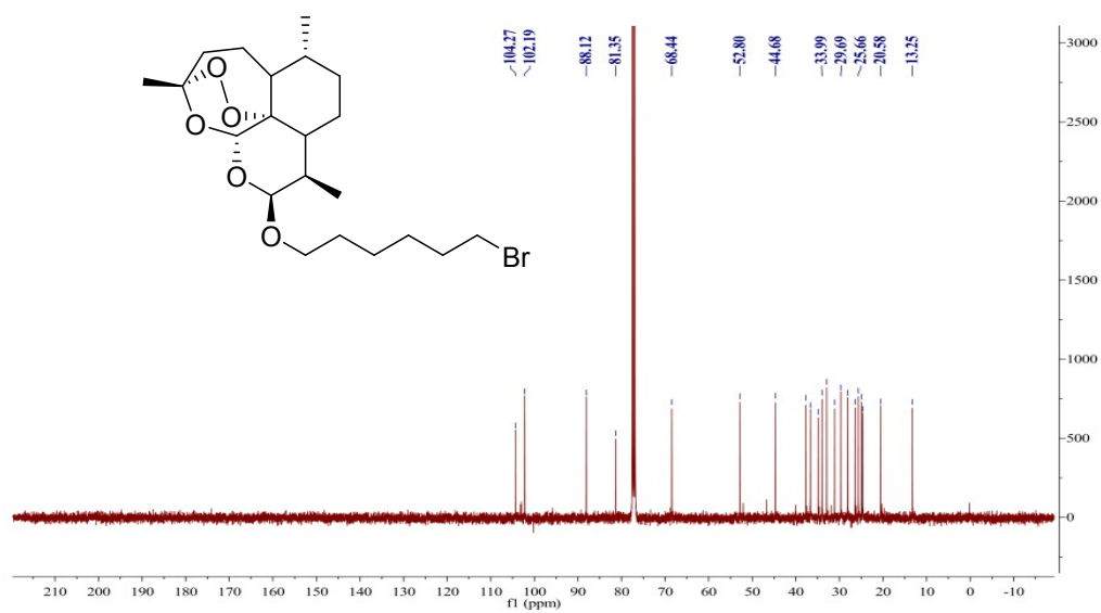
Figure S3. ^1\text{H} NMR spectrum of compound 3c
