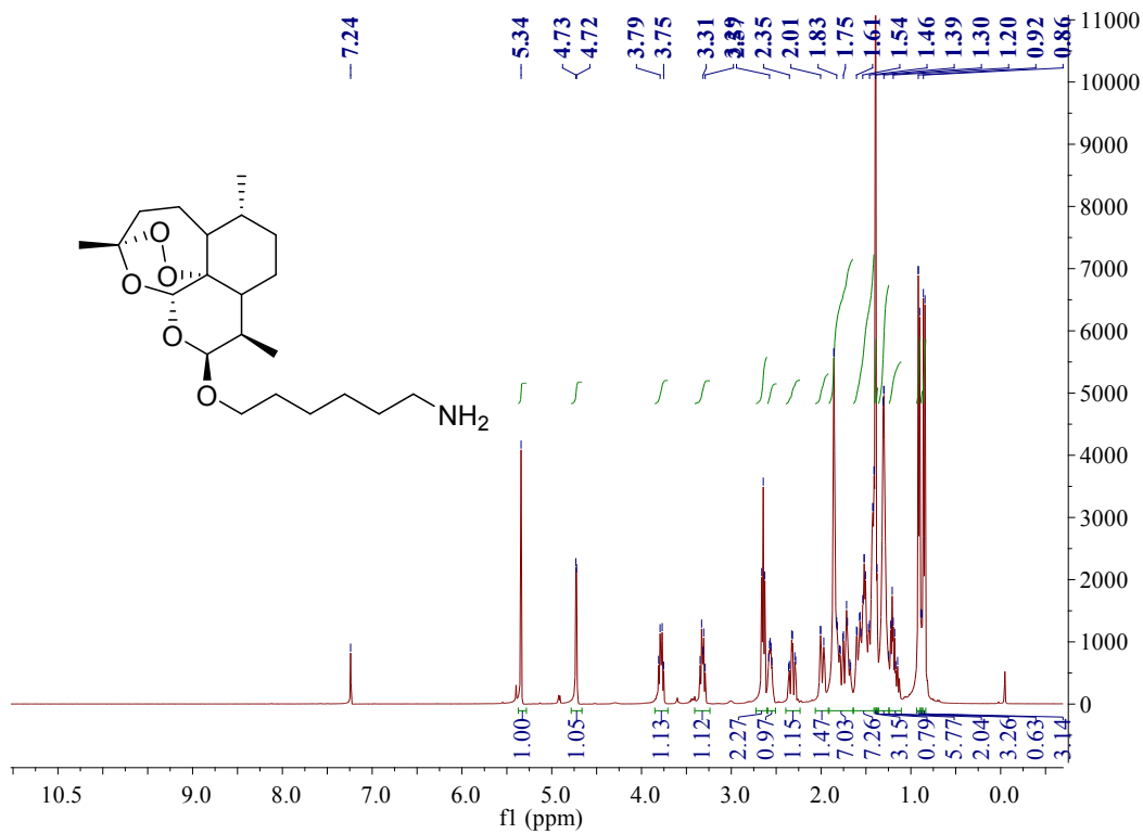
Figure S13. 1 H NMR spectrum of compound 4c
