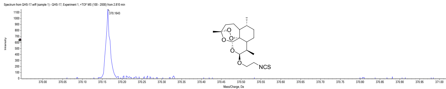
Figure S24. HR-ESI-MS of compound 5a
