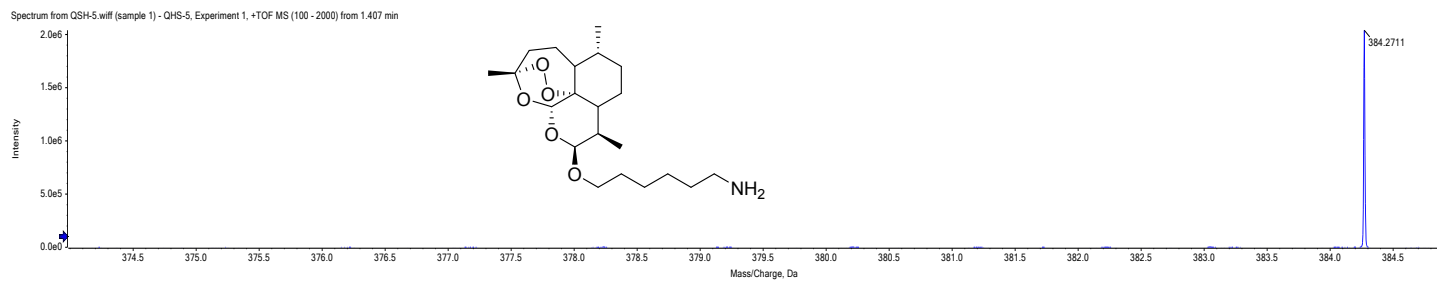
Figure S22. HR-ESI-MS of compound 4b
