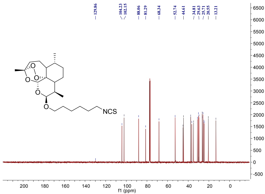
Figure S20. ^{13}\text{C} NMR spectrum of compound 5c
