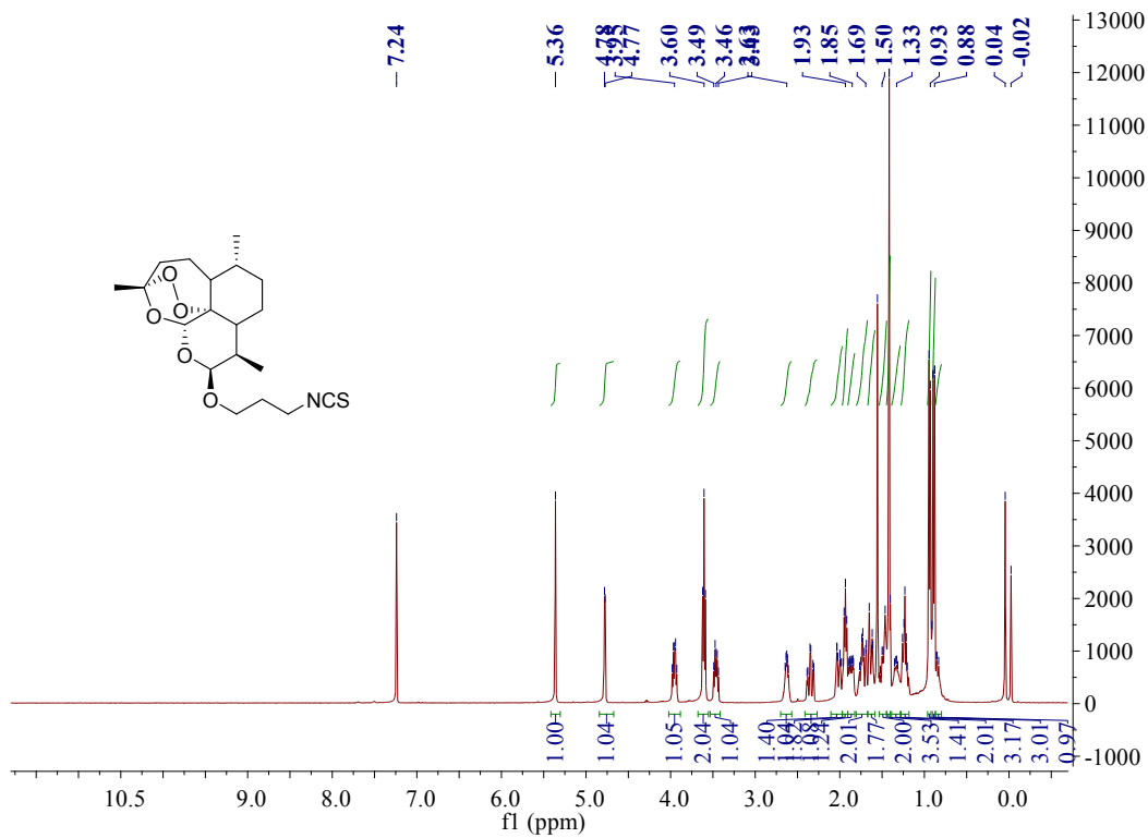
Figure S17. 1 H NMR spectrum of compound 5b
