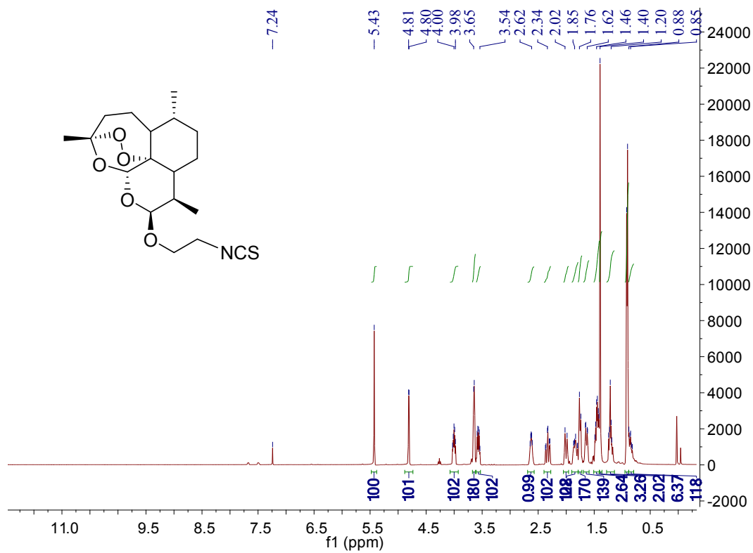
Figure S15. ^1\text{H} NMR spectrum of compound 5a
