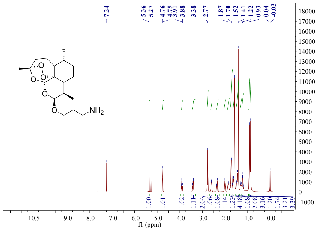
Figure S11. 1 H NMR spectrum of compound 4b
