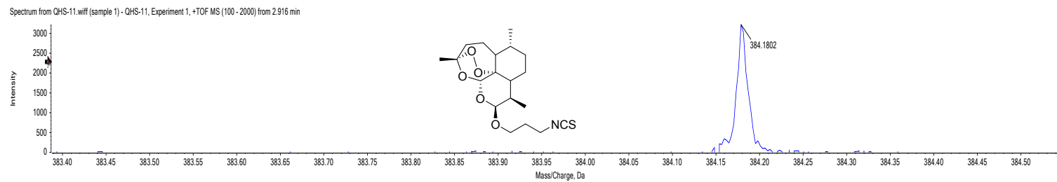
Figure S25. HR-ESI-MS of compound 5b
