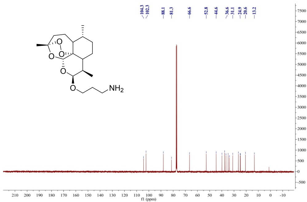
Figure S12. 13 C NMR spectrum of compound 4b
