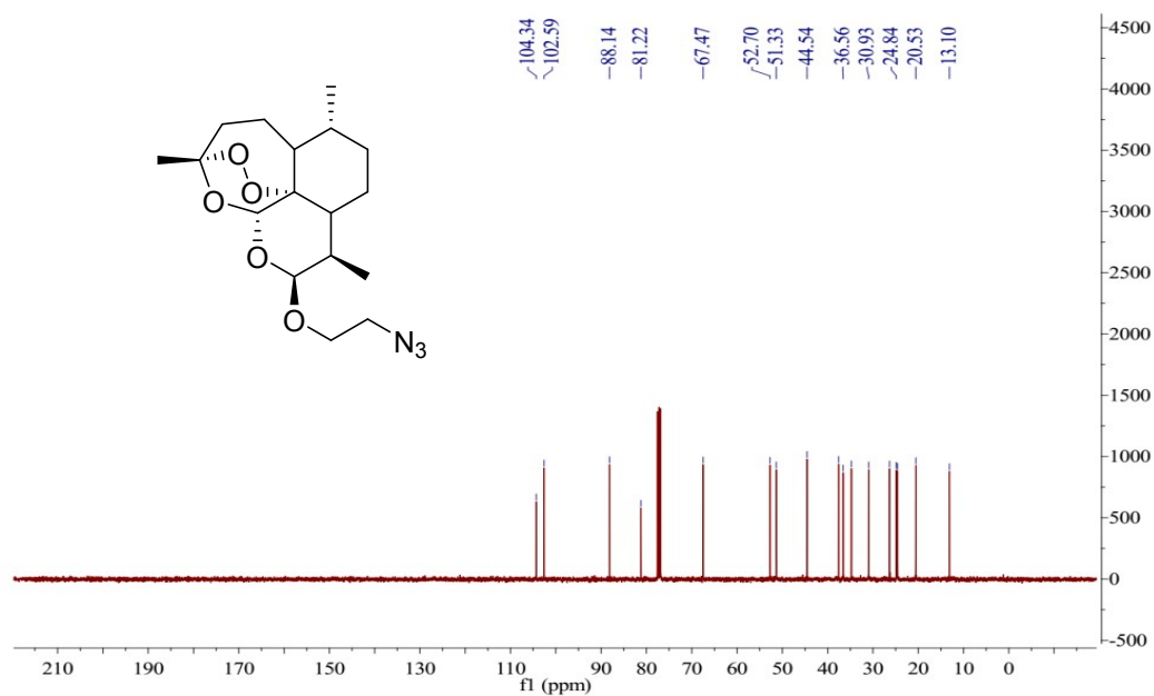
Figure S5. 13 C NMR spectrum of compound 3a
