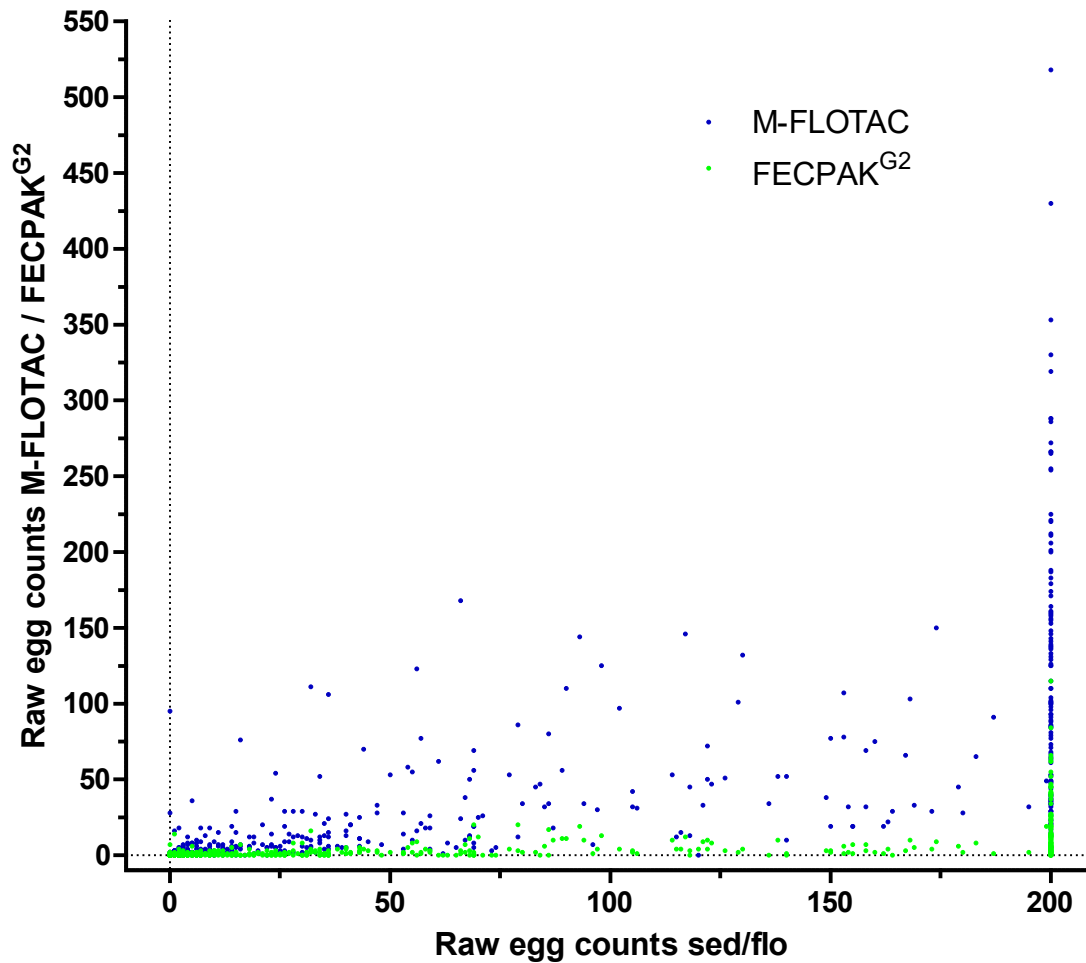
Additional file 2: Figure S1 Comparison of strongyle raw egg counts between semi-quantitative and quantitative methods. The scatter plot shows raw number of eggs counted in the semi-quantitative sedimentation/flotation (sed/flo) on the abscissa compared to raw egg counts obtained with the quantitative Mini-FLOTAC (M-FLOTAC, blue) and FECPAK G2 (green) methods on the ordinate. In the sedimentation/flotation approach, counting was stopped once 200 eggs had been identified.
