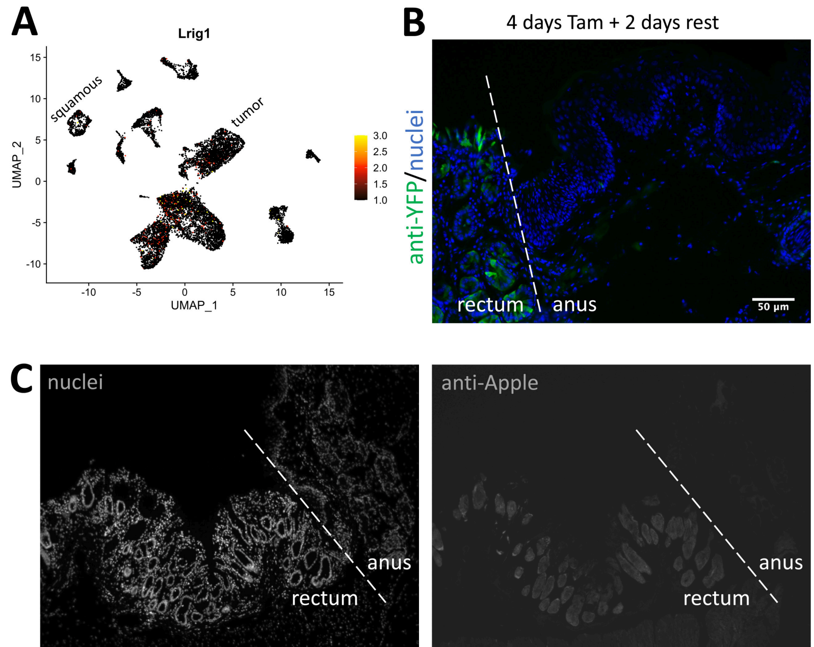
Supplementary Figure S9 | Lrig1 is not expressed in squamous cells. (A) Lrig1 expression in scRNA-seq data of wildtype, APC adjacent, APC tumor, and AOM/DSS tumor samples displayed as a UMAP overlay. Squamous and tumor cell clusters are labeled. (B) Representative IF image from lineage traced Lrig1CreERT2/+; RosaYFP/+ mice. YFP signal was visualized with an anti-YFP antibody, and nuclei are stained with Hoechst. (C) Representative IF image from Lrig1Apple/+ reporter mice. Apple signal was visualized with an anti-Apple antibody (right), and nuclei are stained with Hoechst (left). For both (B) and (C) , colon and anus were collected, and the anorectal junction is depicted by the dashed line. Magnification is the same for all images.
