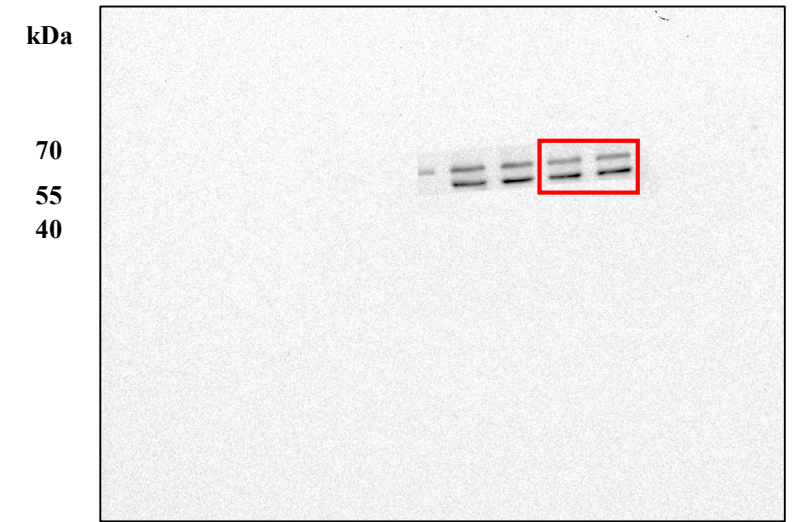
Anti-T- JNK
