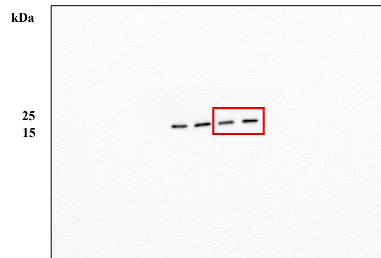
Anti-BAX
