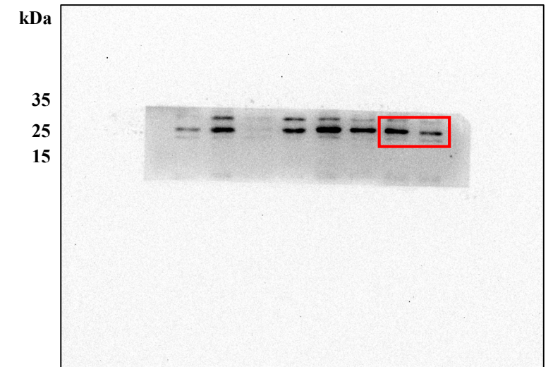
Anti-BCL-2
