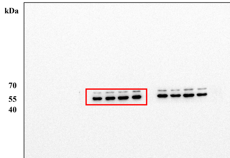
HT29 Anti-T-JNK
