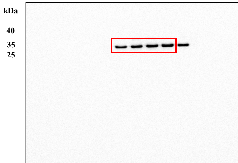
HCT116 Anti-GAPDH
