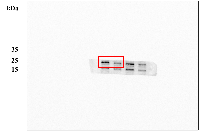
Anti-BCL-2
