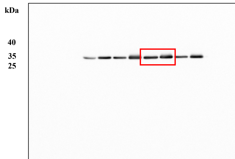
HCT116 Anti-BAX
