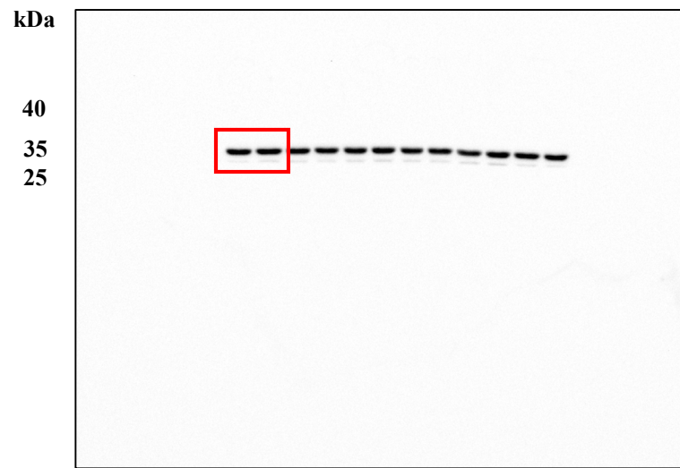
HT29 Anti-GAPDH
