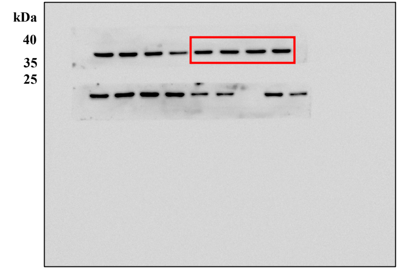
Anti-GAPDH
