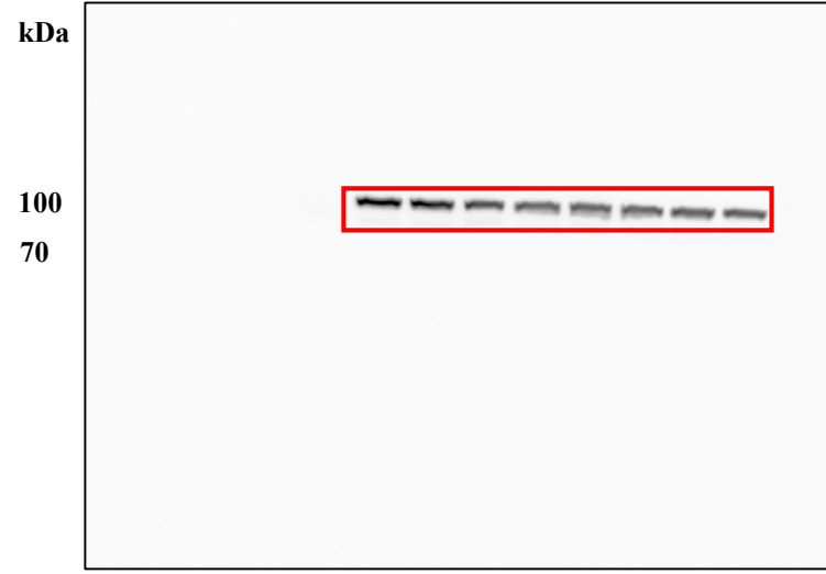
Anti-HSP90AA1
