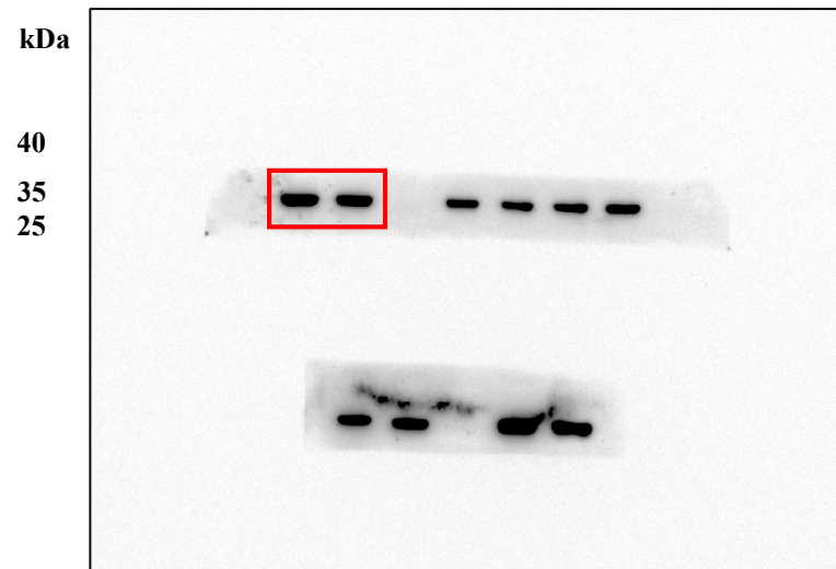
HT29 Anti-GAPDH
