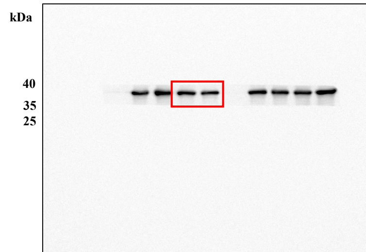
Anti-GAPDH
