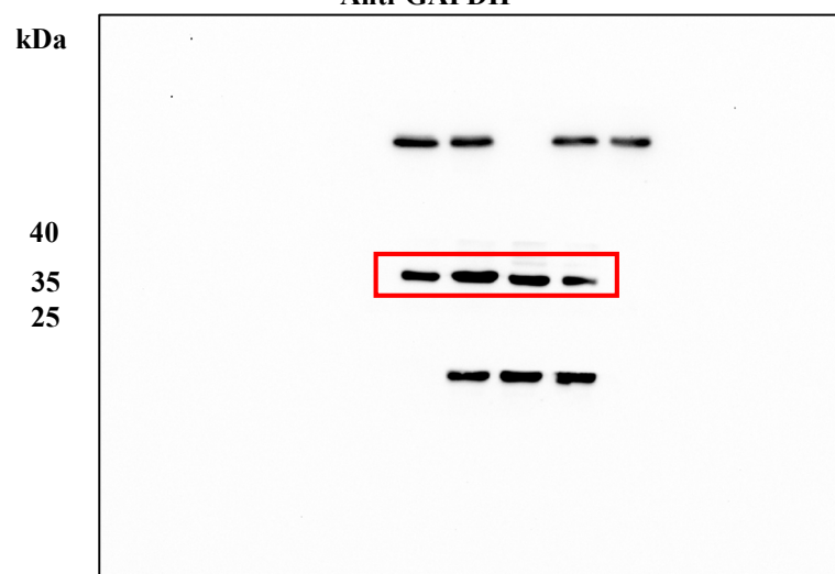
Anti-GAPDH
