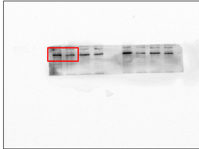
Anti-BCL-2
