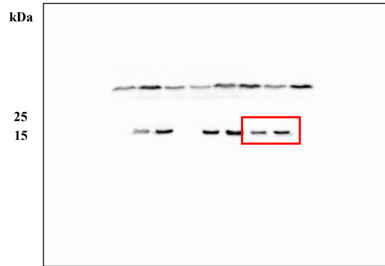
HCT116 Anti-BAX
