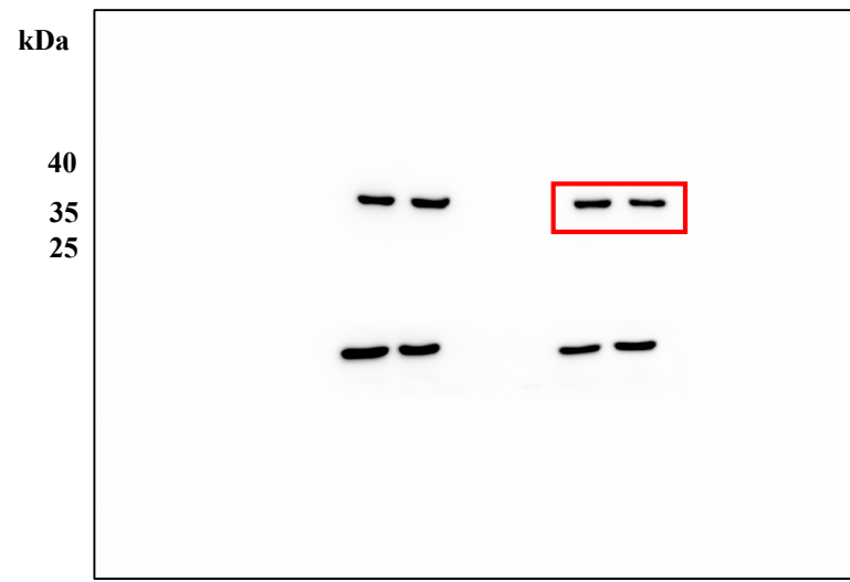
Anti-GAPDH
