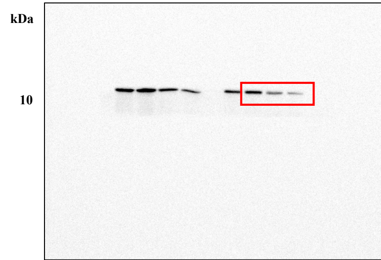
HCT116 Anti-SRP9
