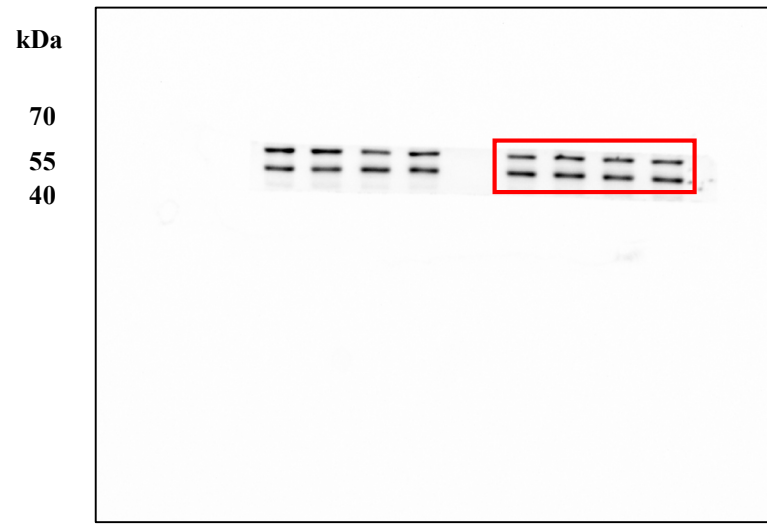
HCT116 Anti-T-JNK
