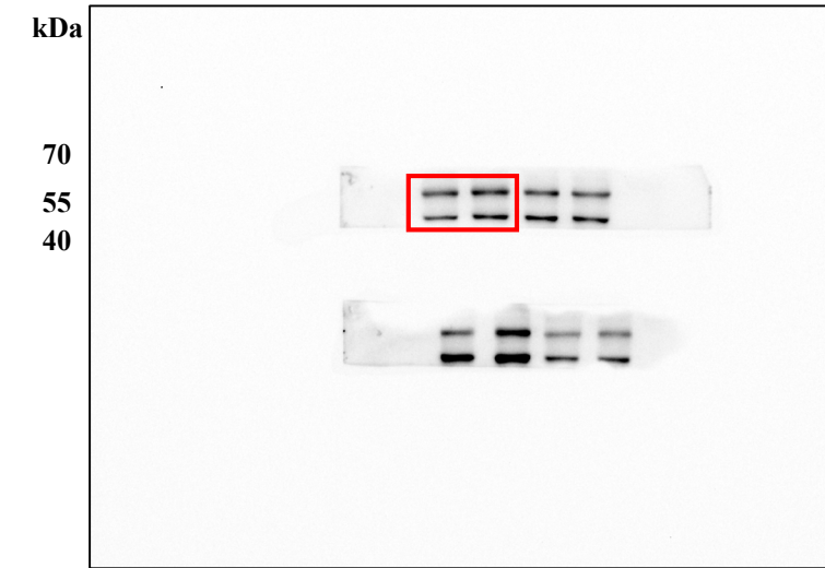
Anti-T- JNK
