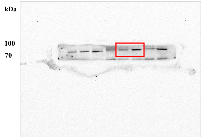
Anti-HSP90AA1
