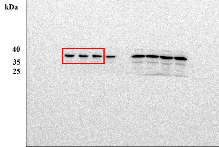
Anti-GAPDH
