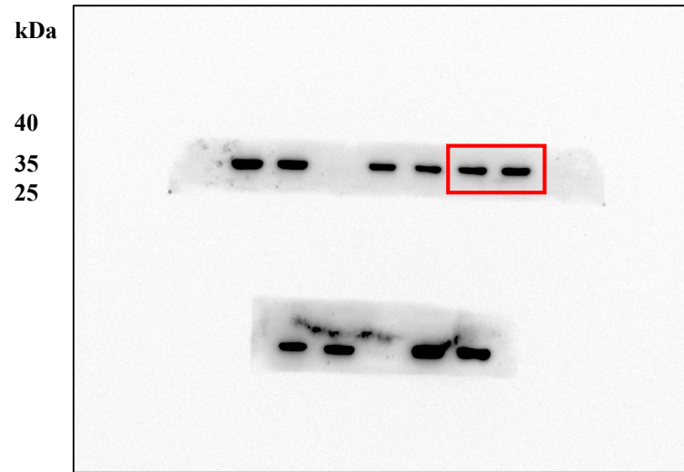
HCT116 Anti-GAPDH
