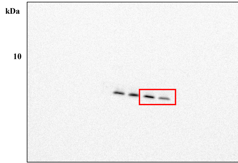
Anti-SRP9
