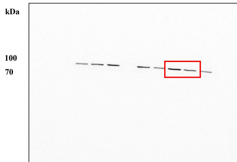
HCT116 Anti-HSP90AA1
