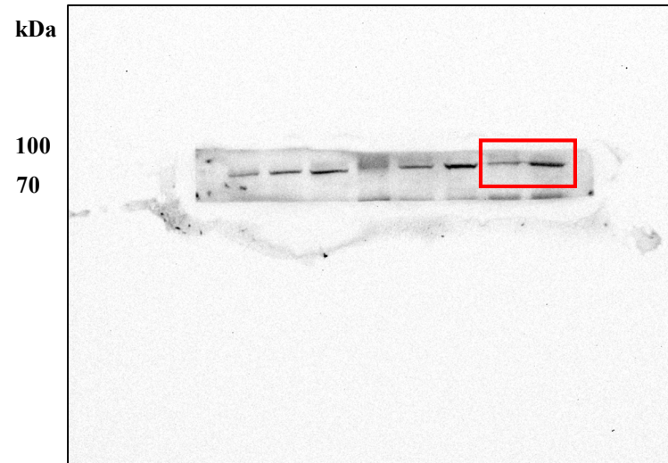
Anti-HSP90AA1
