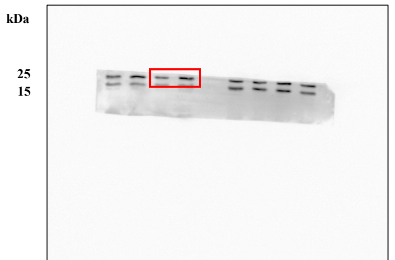
Anti-BAX
