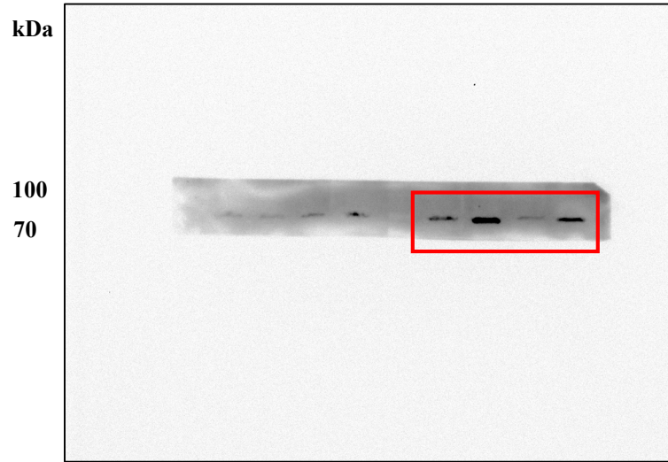
Anti-HSP90AA1
