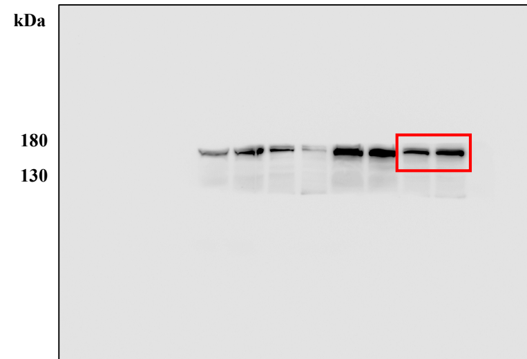
Anti-T-ASK1
