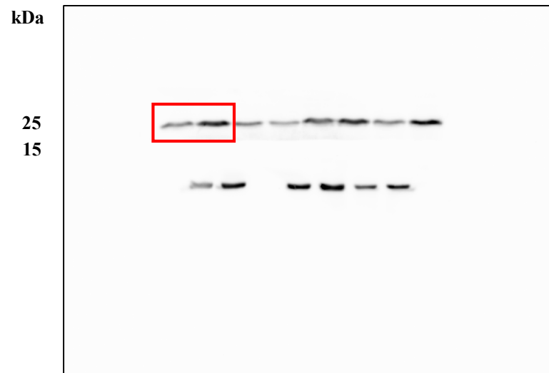
HT29 Anti-BAX
