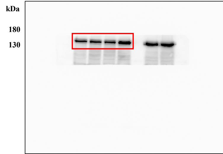
Anti-T-ASK1
