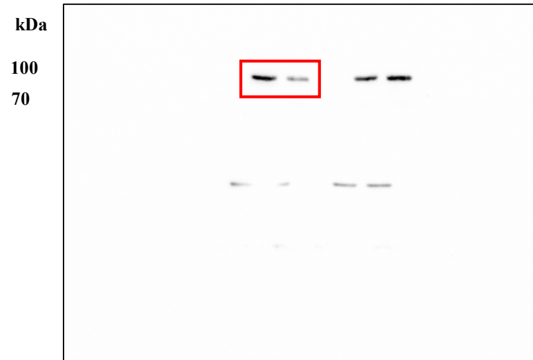
HT29 Anti-HSP90AA1
