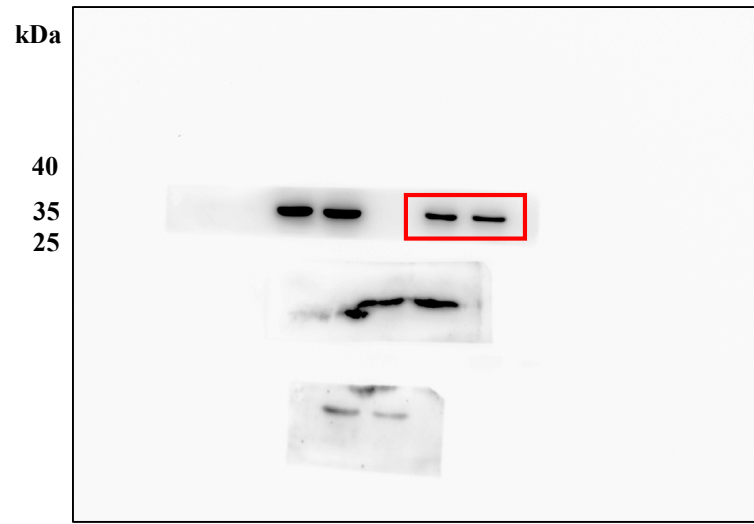
Anti-GAPDH
