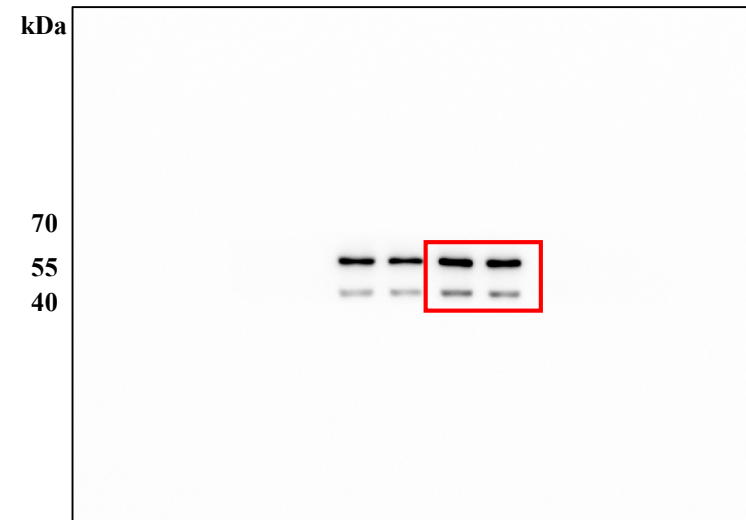
Anti-T- JNK
