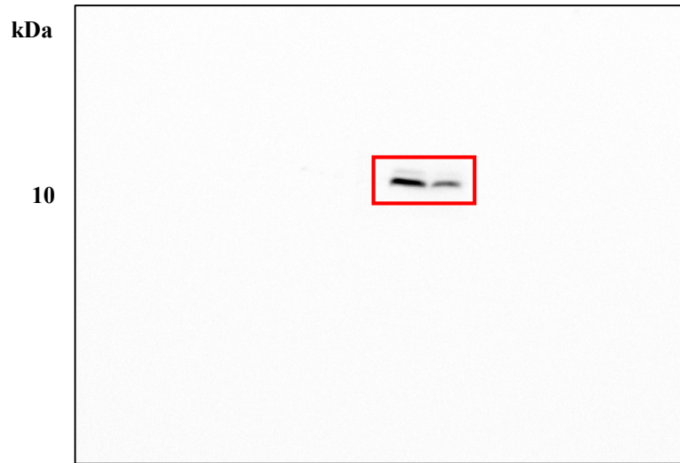
Anti-SRP9
