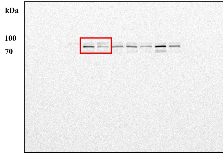
HT29 Anti-HSP90AA1
