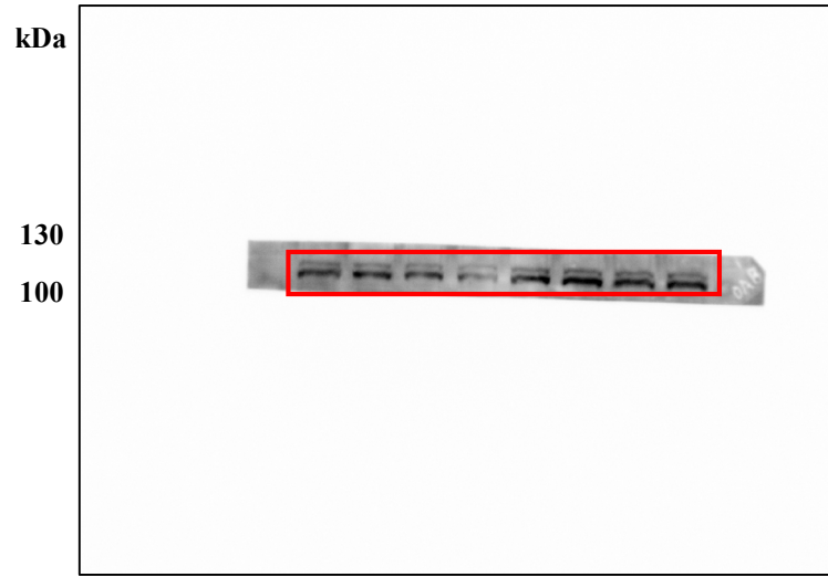
Anti-DAB2IP
