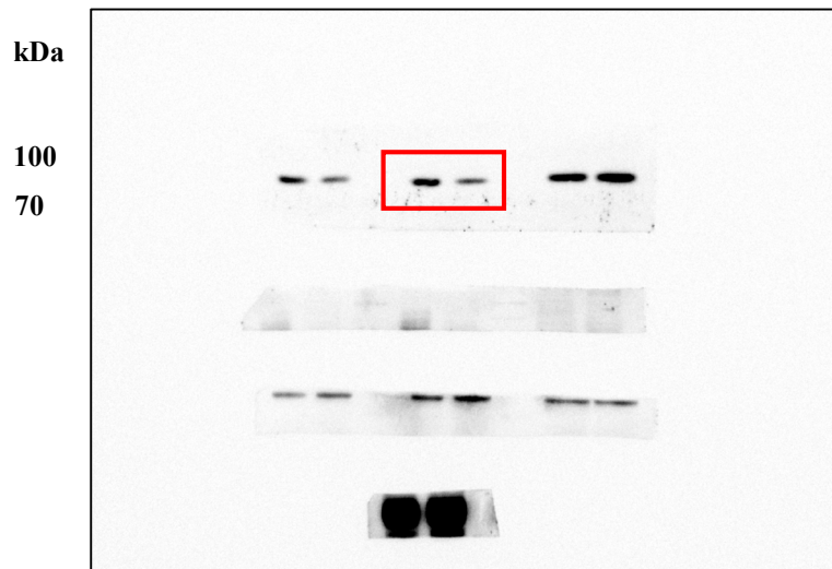
HCT116 Anti-HSP90AA1
