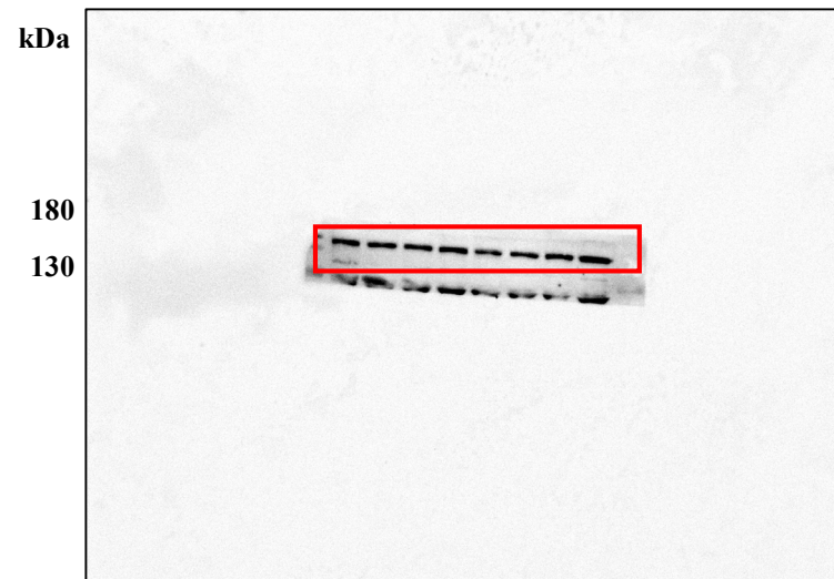
Anti-T-ASK1
