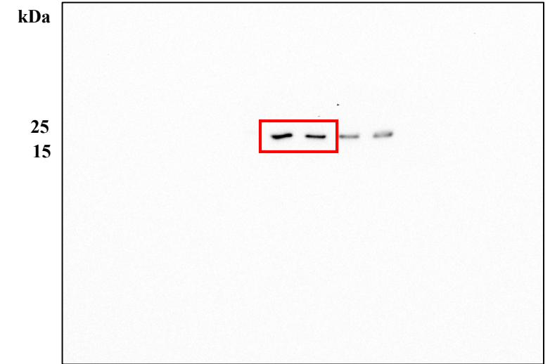
Anti-BAX
