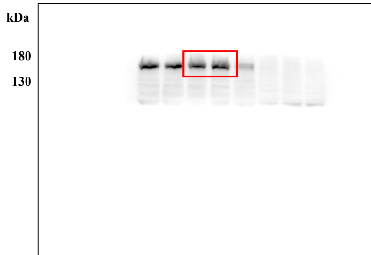
Anti-T-ASK1
