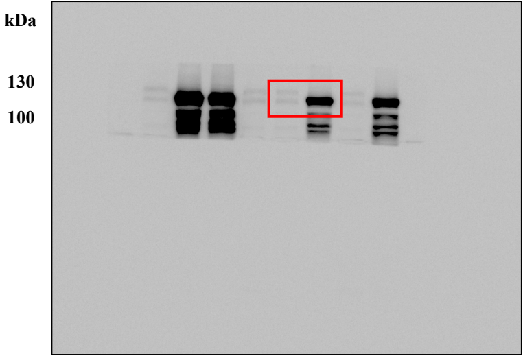
Anti-DAB2IP
