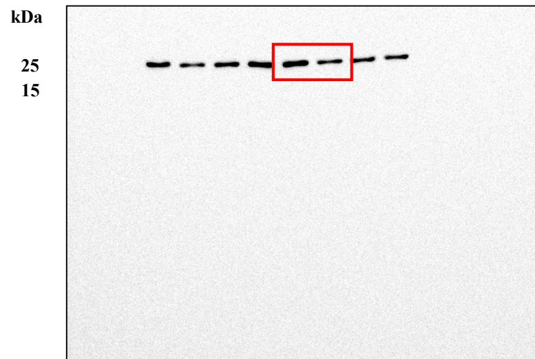
HT29 Anti-BAX
