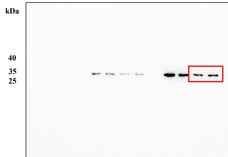
HCT116 Anti-GAPDH
