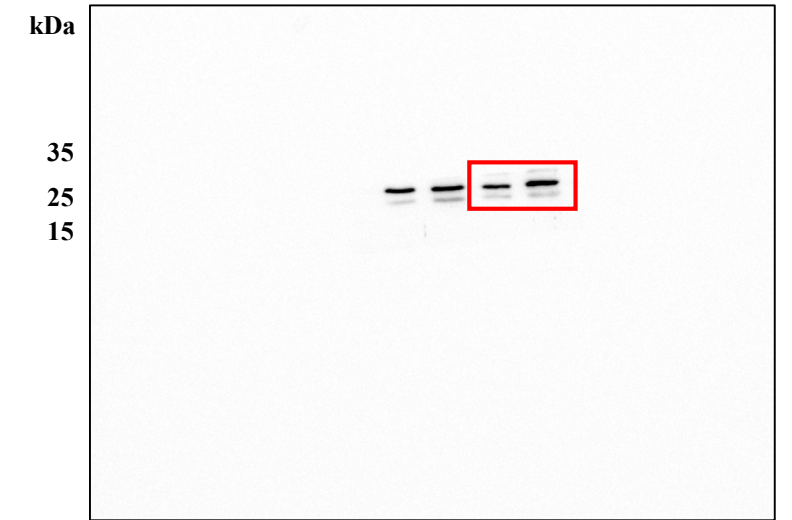
Anti-BCL-2
