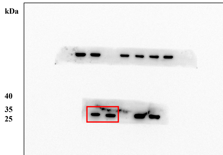
HCT116 Anti-GAPDH
