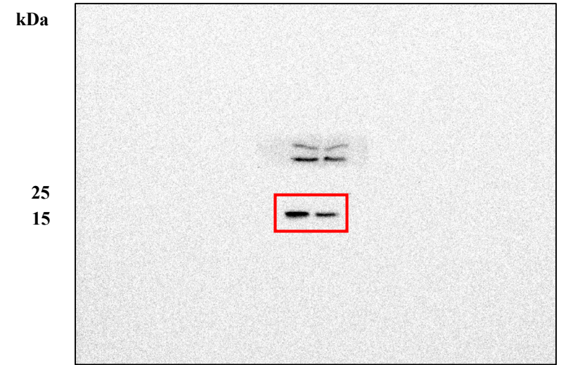
Anti-BAX
