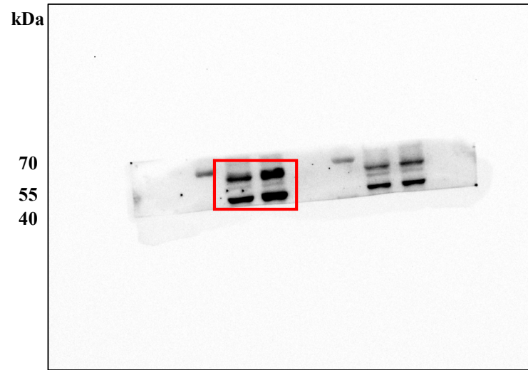
Anti-T- JNK
