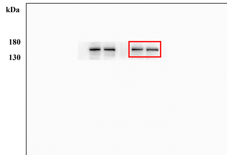
Anti-T-ASK1
