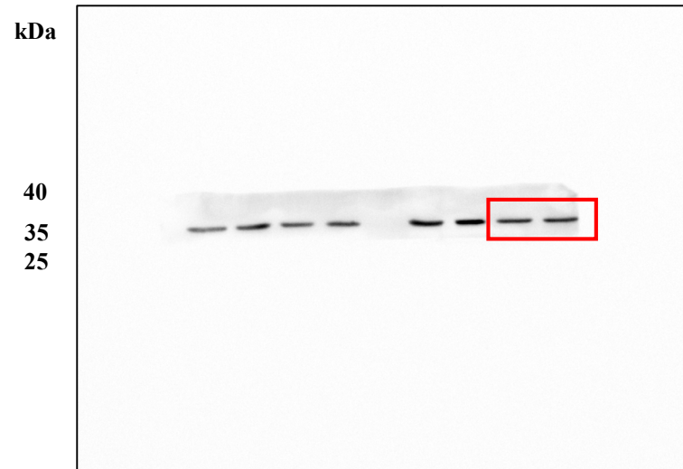
HCT116 Anti-GAPDH
