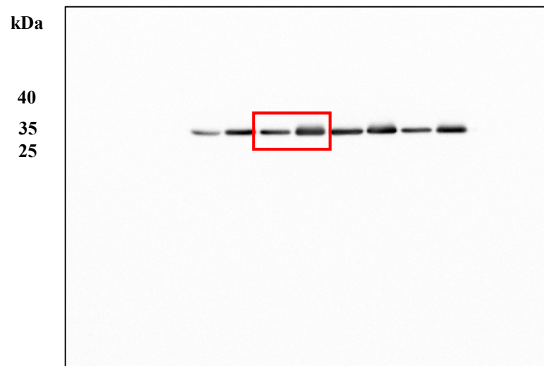
HT29 Anti-BAX
