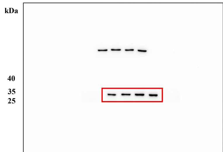
HT29 Anti-GAPDH
