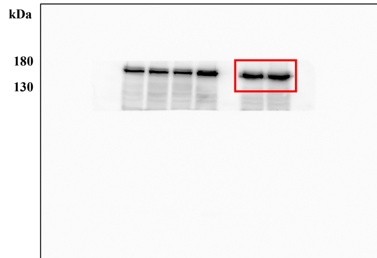
Anti-T-ASK1
