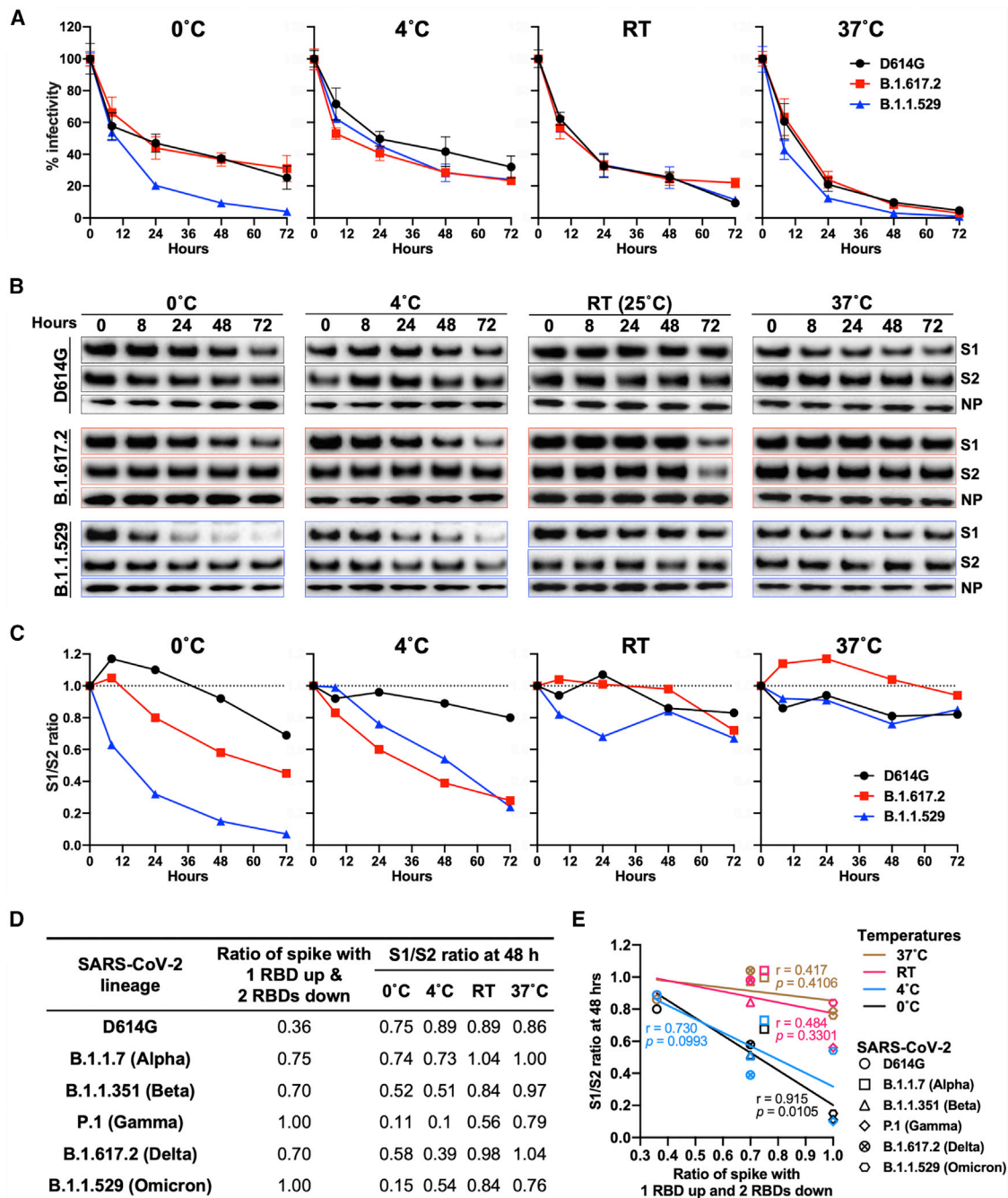
Figure 4. Stability of SARS-CoV-2 D614G, B.1.617.2, and B.1.1.529 spikes at different temperatures
