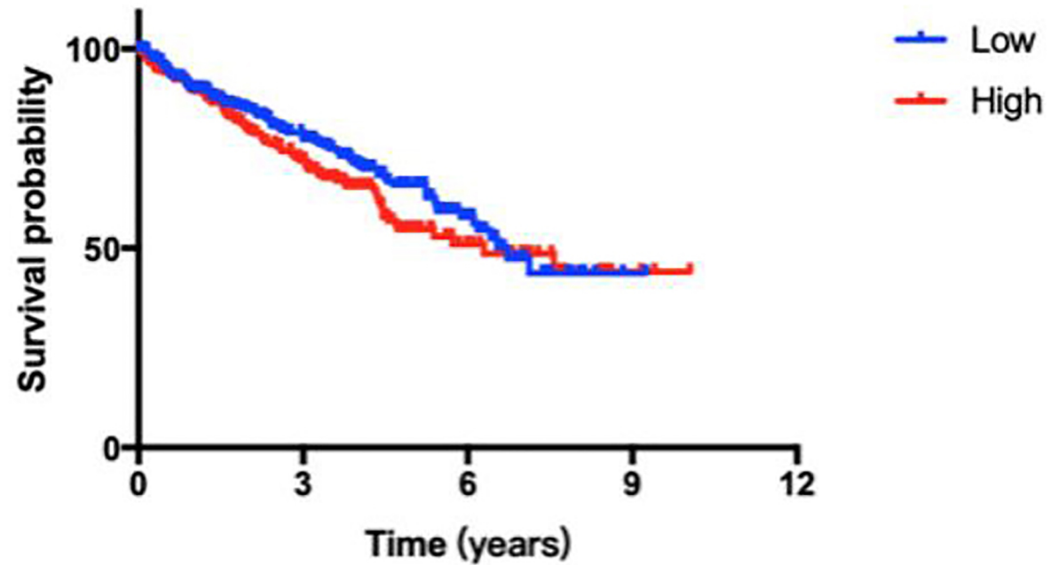
NPC1 (p=0.207)
