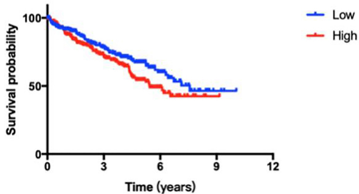
CDKN2A (p=0.053)
