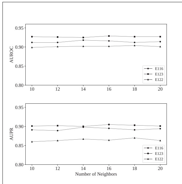
Figure S1: Effect of number of neighbors on classification performance. The performance of the model on the classification task is plotted as a function of the number of neighbors subsampled for each genic node. Including additional neighbors beyond 10 does not lead to substantial performance improvements with respect to either (a) AUROC or (b) AUPR.
