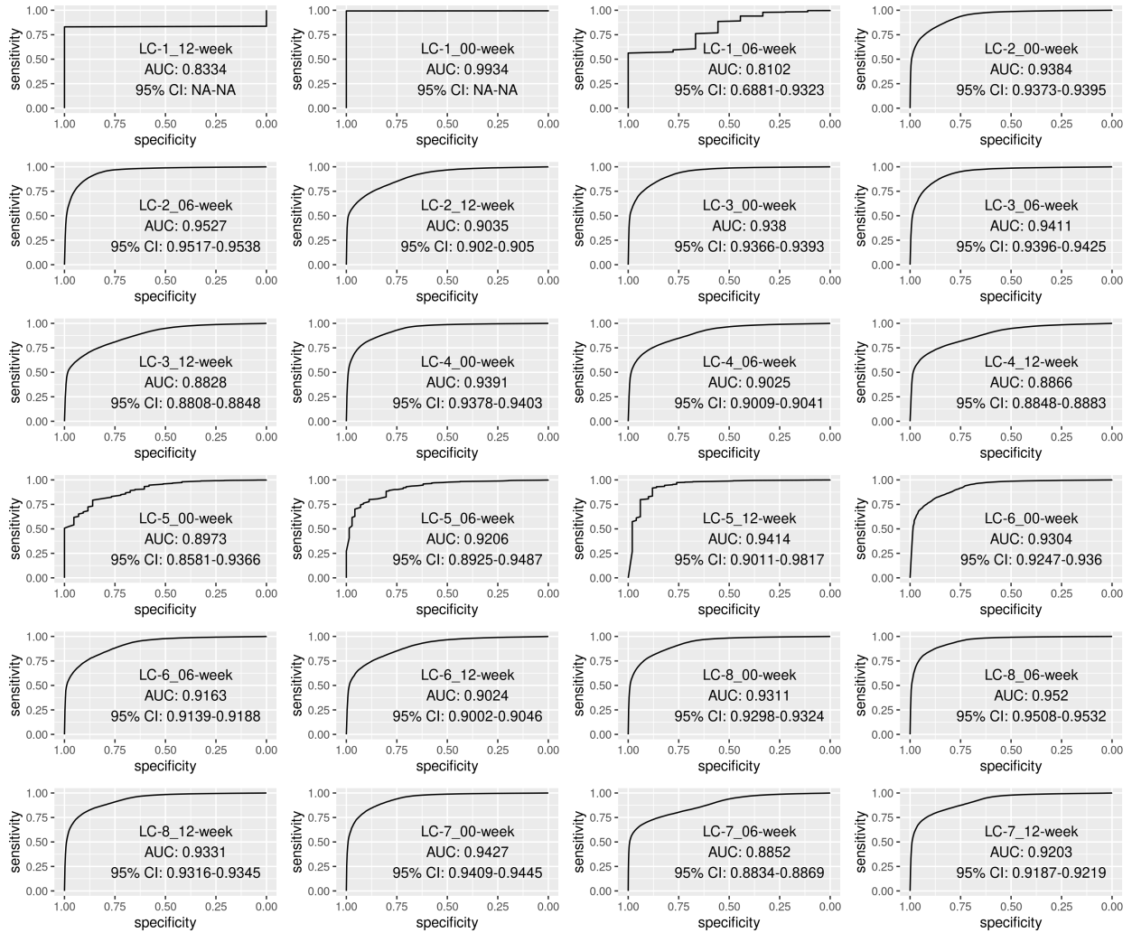
Figure S5. Performance of the random forest model in the 24 independent testing datasets from 8 NSCLC patients. The receiver operating characteristic (ROC) curve of the random forest model in the 24 independent datasets.
