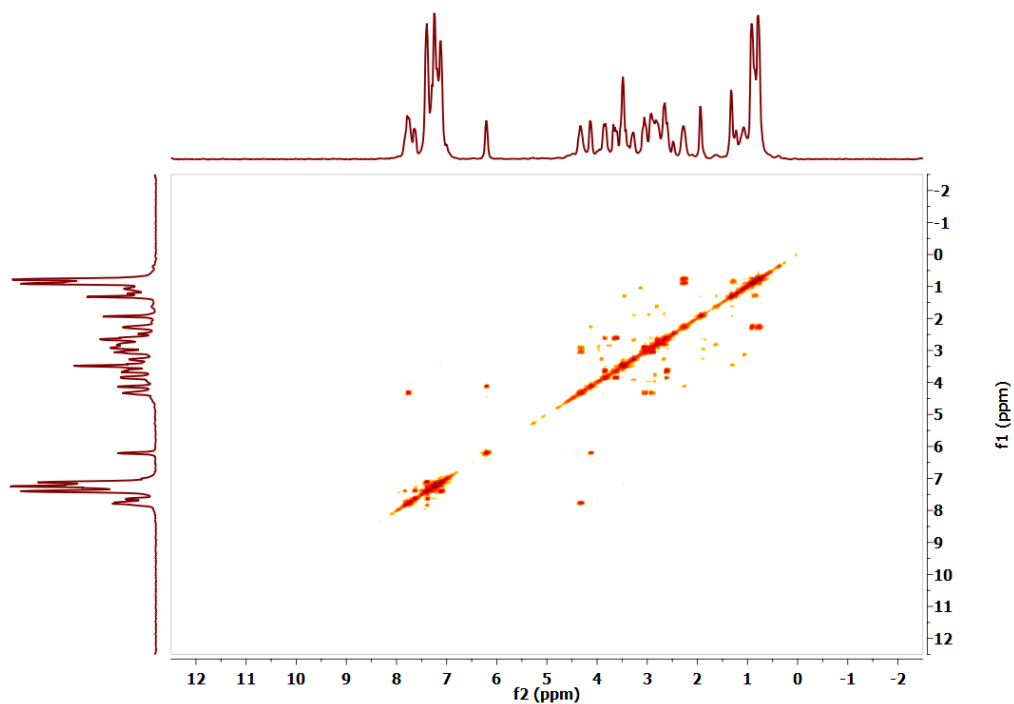
Fig S5. 2D COSY NMR of Compound 2 in CDCl 3 .
