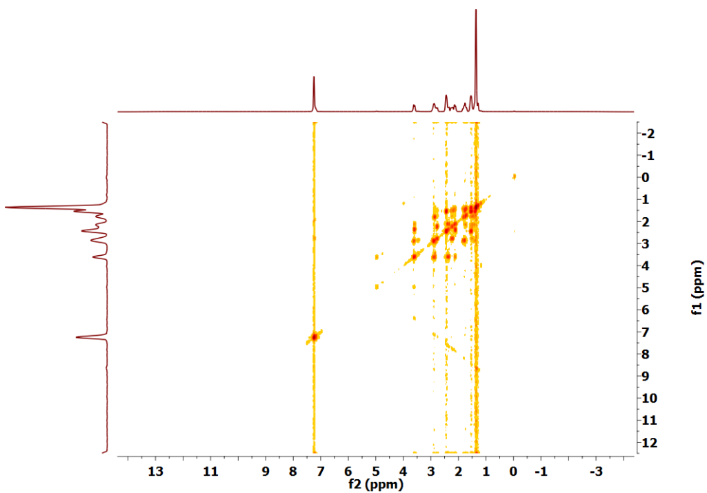
Fig S3. 2D COSY NMR spectra of compound 1 in CDCl 3 .
