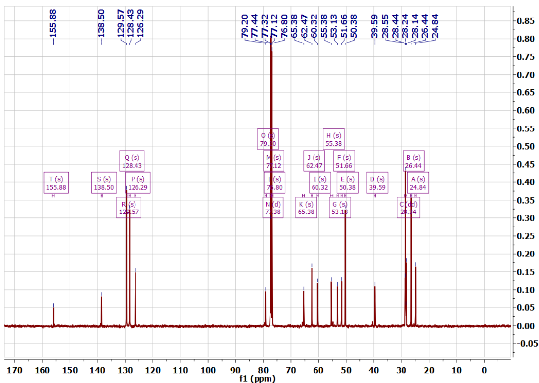
Fig S2. 13 C NMR spectra of compound 1 in CDCl 3 .
