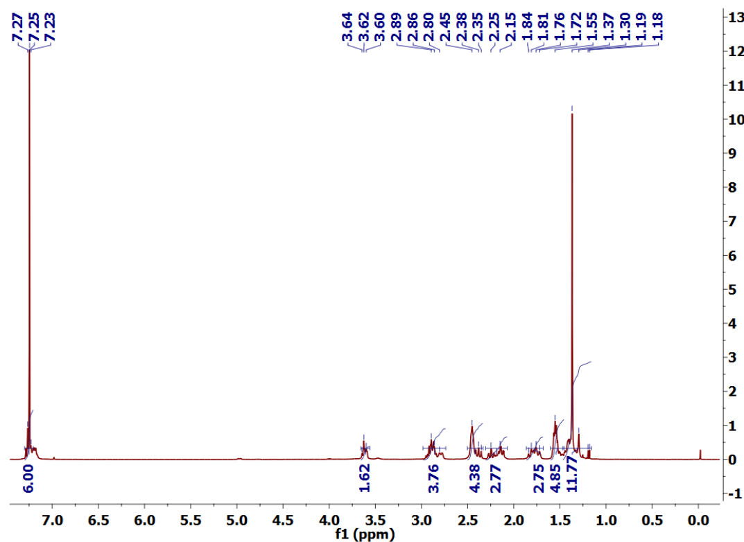
Fig S1. 1 H NMR spectra of compound 1 in CDCl 3 .
