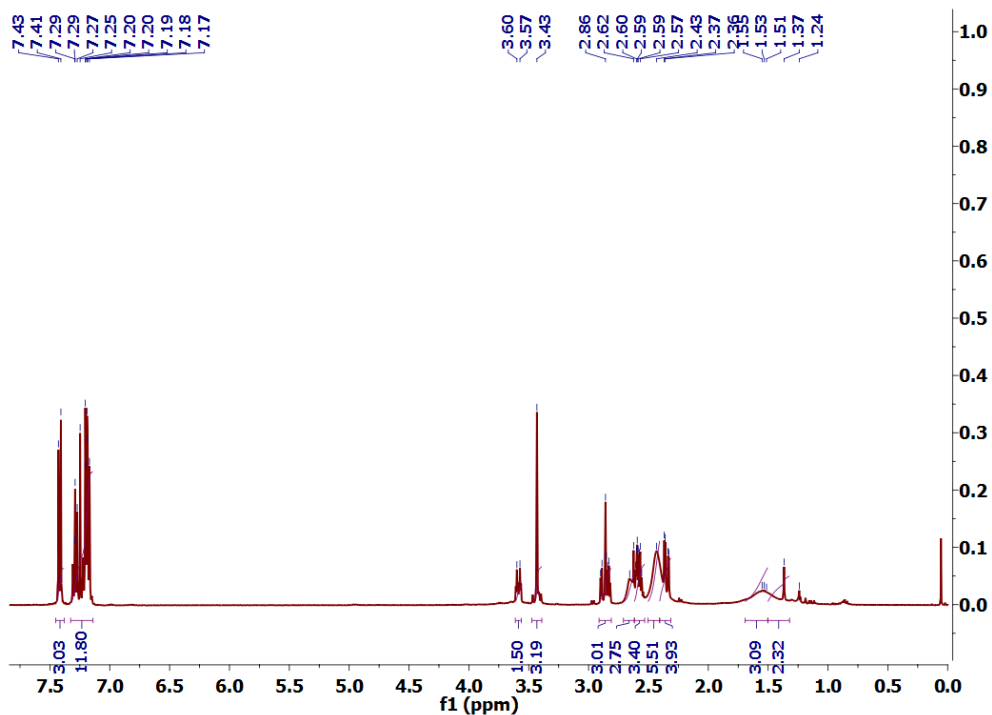
Fig S4 1 H NMR spectra of compound 2 in CDCl 3 .
