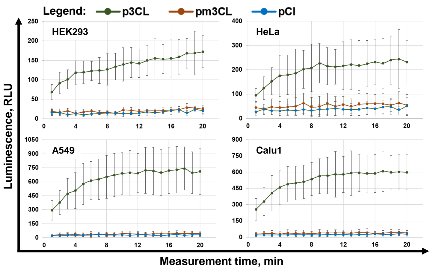
S2 Fig. 3CL pro proteolytic activity analysis. Cells were co-transfected with p3CL, pm3CL, or pCI constructs and pGlo-3CL providing the expression of 3CL pro -specific biosensor; 24 h post transfection luciferase activity in transfected cultures was analyzed using GloSensor reagent. Values are represented as mean \pm SD of two independent experiments with triplicates (n = 6).
