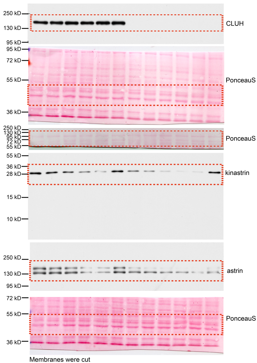
Figure 2A WT CLUH KO CHX [h] 0 2 4 6 8 8 0 2 4 6 8 8 MG132 - - - - - + - - - - - +
