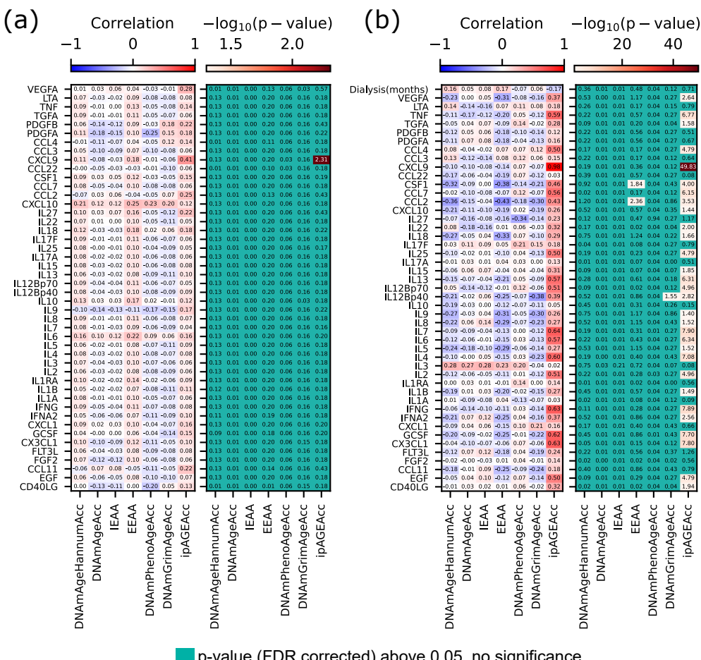
Supplementary Figure 5. Association of inflammatory/immunological proteins with different types of age acceleration. (a) Pearson correlation coefficients and corresponding FDR-corrected p-values resulting from the correlation of protein levels and each type of age-acceleration, in the control and (b) ESRD groups. (c) Table with the number of proteins significantly associated with different types of age acceleration (FDR-corrected Pearson correlation p-value below 0.05). (d) Venn diagram of ESRD-associated, chronological age-associated inflammatory/immunological proteins in the control group and ipAGE acceleration associated in ESRD group. (e) Association between CXCL9 and ipAGE acceleration.
