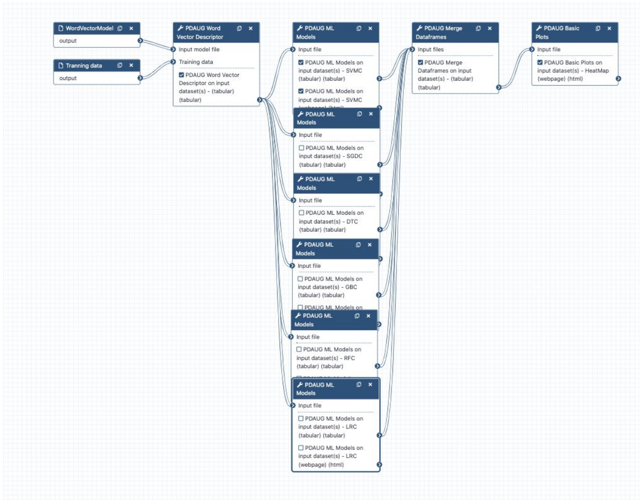
Supplementary Figure 1. Workflow to perform machine learning modeling based on word vector descriptors.
