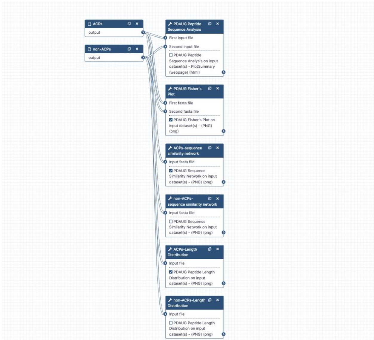
Supplementary Figure 3. Workflow to generate summary plot, Fisher's plot, sequence similarity network, and length distribution plot.
