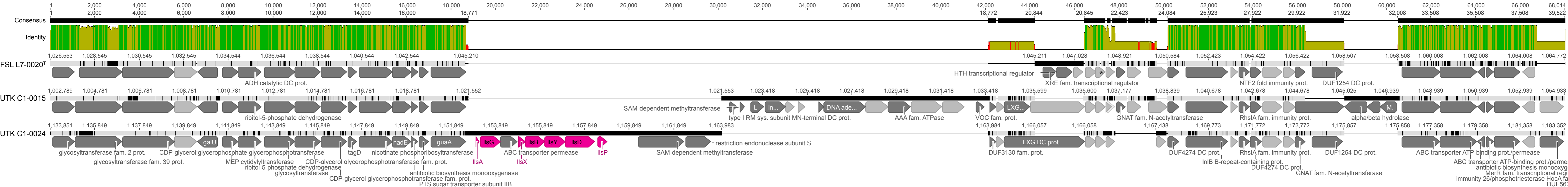
Supplementary Figure S1. Listeria pathogenicity island 3 (LIPI-3) in UTK C1-0024
