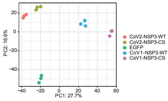
PCA plot of top 1000 variable GlyGly (K)Sites
