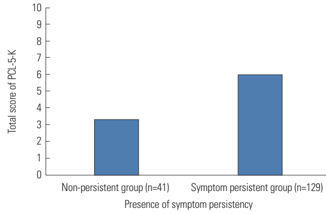
Supplementary Fig. 4. Total scores for PCL-5-K in the symptom persistent and non-persistent groups. PCL-5-K, Korean version of Posttraumatic Stress Disorder Checklist-5.
