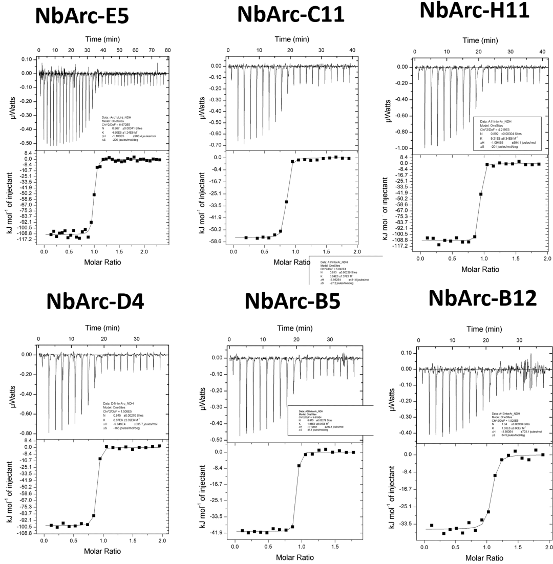
S2 Figure. NbArc ITC titrations into FLrArc-7A, raw and integrated thermograms.
