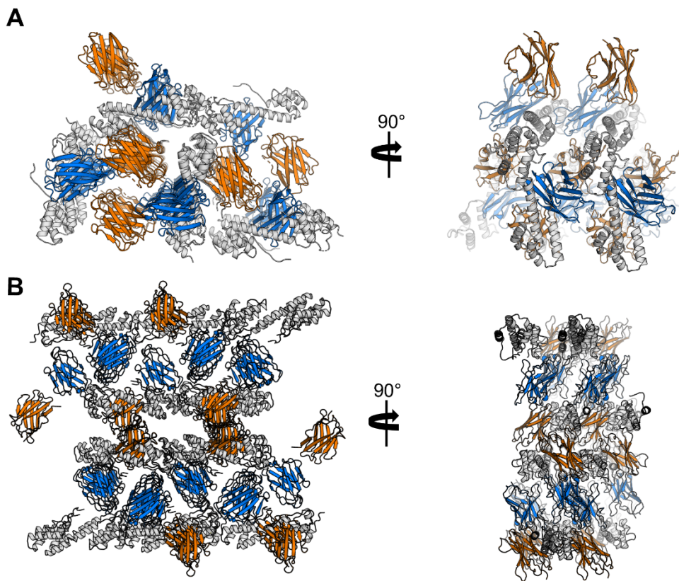
S4 Figure. Crystal contacts. In both the rArc-CTD ( A ) and the hArc-CTD extended crystal structure ( B ), contacts were formed almost exclusively by the bound Nbs. The CTD is coloured grey, H11 orange and C11 blue.
