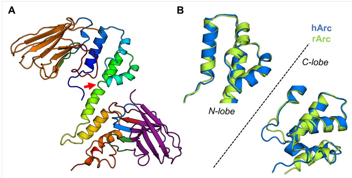
S5 Figure. Crystal structure of hArc-CTD in complex with NbArc-H11 and -C11. A The structure of the ternary complex. The breaking of the central helix of the CTD is highlighted with a red arrow. The hArc-CTD is coloured blue to red from N- to C-terminus. H11 is shown in orange and C11 in purple. CDR 1, 2, and 3 are coloured blue, green, and red, respectively. B Superimposition of the N- and C-lobes of rArc and hArc CTD from the crystal structures.
