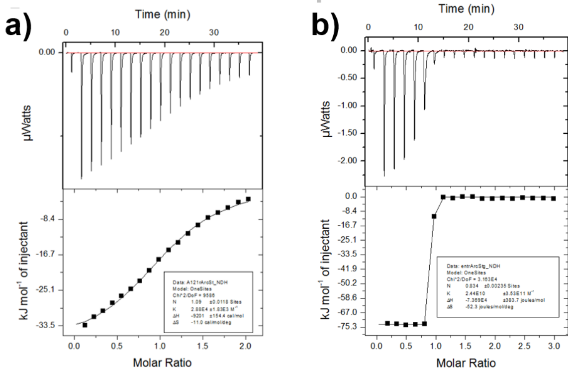
S6 Figure. Raw ITC thermograms. A Titration of the Stg peptide into FLrArc-7A. B titration of NbArc-H11 into Stg-bound FLrArc-7A.
