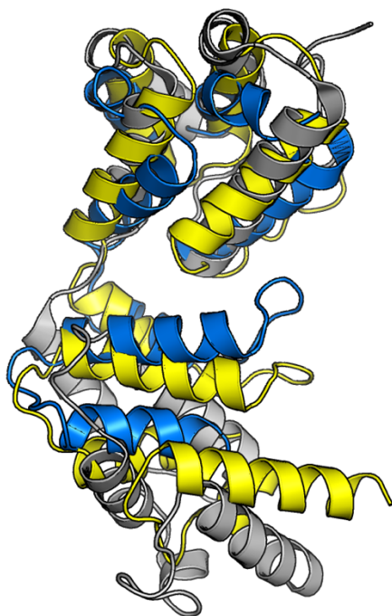
S13 Figure. Superposition of collapsed conformations. The collapsed hArc CTD crystal structure (blue), dArc2 monomer from a capsid (gray), and AlphaFold2 prediction of the collapsed form (yellow).
