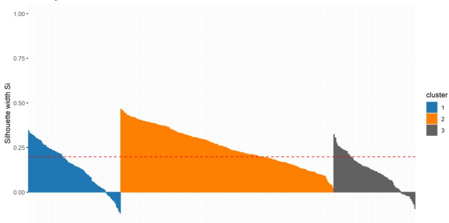
Clusters silhouette plot Average silhouette width: 0.2
