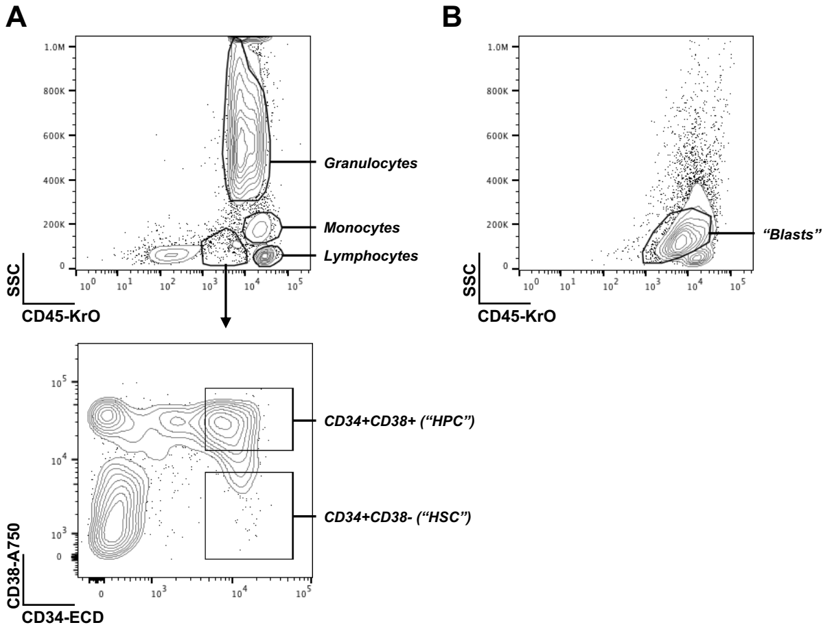
Supplementary Figure S2. Gating of subpopulations for FACS validation of putative Surfaceome targets. A: Expression of putative Surfaceome markers was assessed on healthy bone marrow specimens gating for both mature (lymphocyte, monocyte, granulocyte) as well as progenitor (hematopoietic stem cell "HSC", hematopoietic progenitor cell "HPC") populations. B: Gating of "Blast" population in leukemia specimens. "Blasts" were gated based on dim/intermediate CD45 expression.
