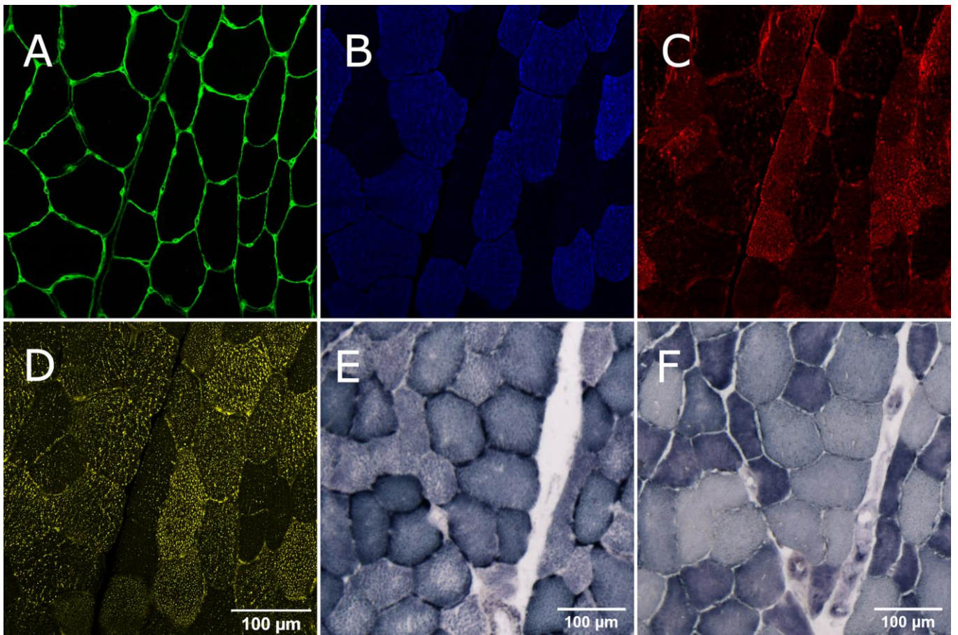
Supplemental Figure 1. Representative staining images. A: Cell borders, B: Type I fibers, C: Type IIX fibers, D: Lipid droplets, E: Succinate dehydrogenase, F: \alpha -glycerophosphate dehydrogenase. Images A-D are layers of a single confocal microscopy image (sections B and C enhanced here only for visual purposes). Images E and F are from sequential sections.
