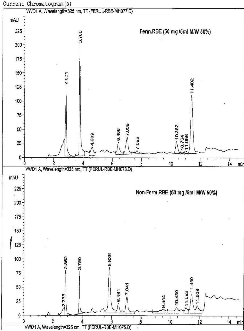
Figure S1. HPLC profiles of the methanolic extracts of fermented (FRBE) and non-fermented rice bran (RBE)
