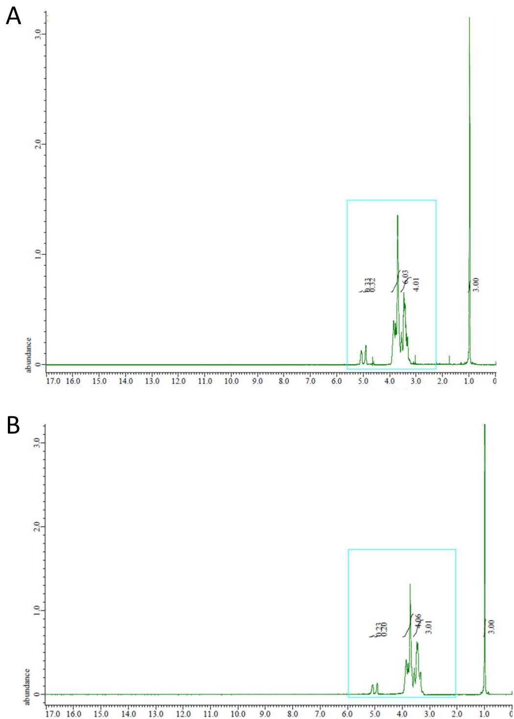
Figure S2. ^1\text{H} NMR spectra of (A) HP \beta CD, and (B) FRBE/HP \beta CD complex.
